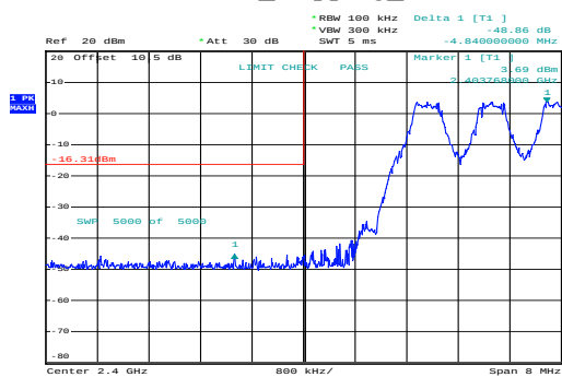
GFSK_Hopping_Lower
