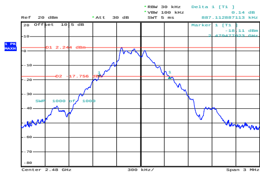
GFSK_High
