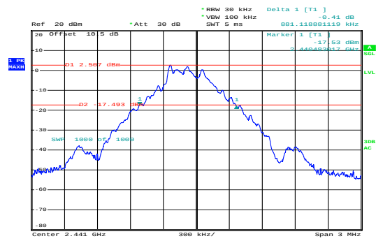
GFSK_Middle
