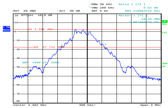
GFSK_Low
