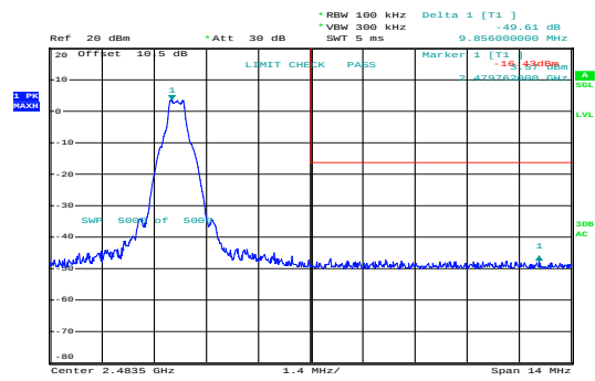
GFSK_High
