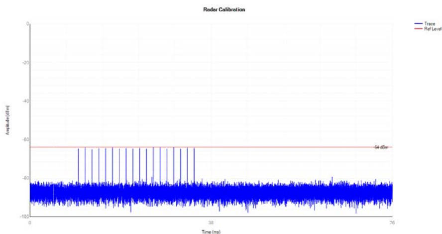
Radar Signal 5260
