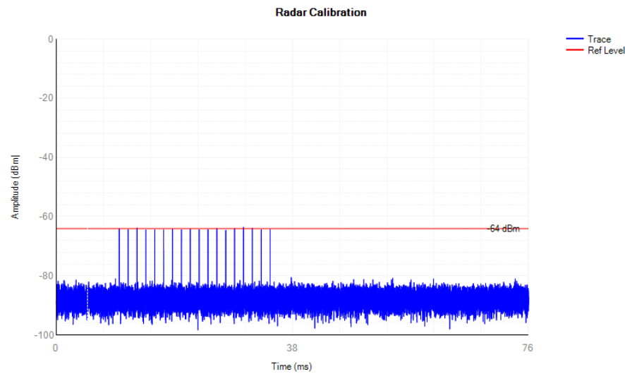
Radar Signal 5530
