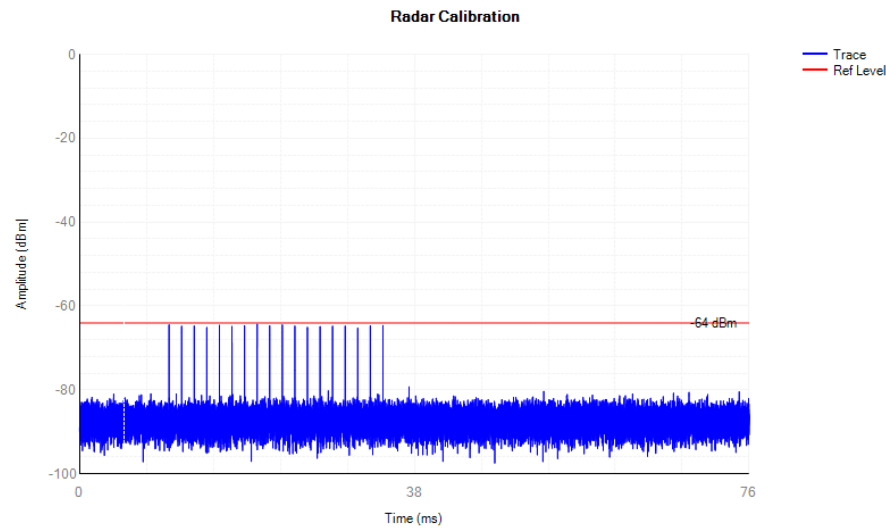
Radar Signal 5290
