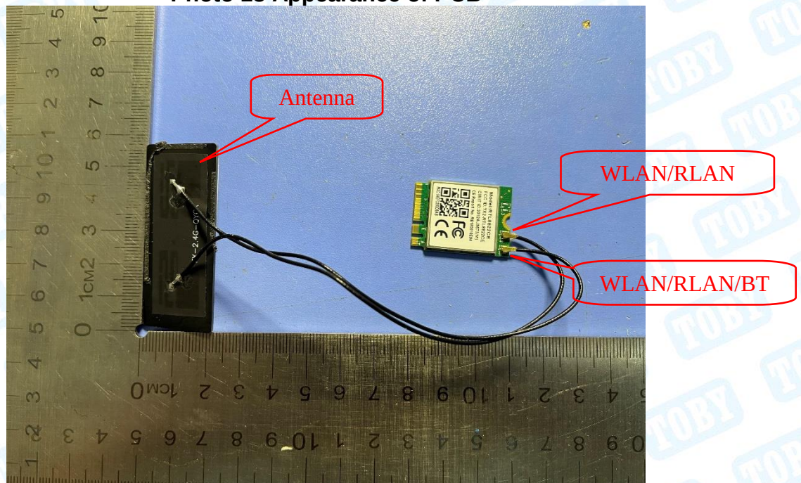
Photo 19 Appearance of PCB
