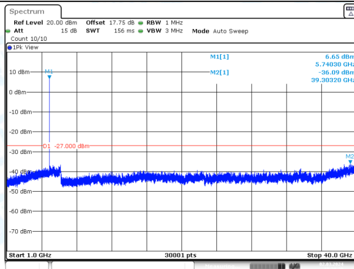
11N20SISO_Ant1_5745_1000~40000
