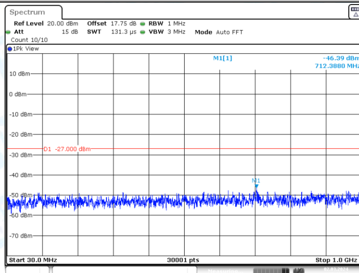
11N20SISO_Ant2_5745_30~1000
