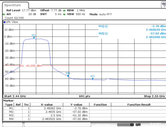
11G_Ant2_High_2462_AV
