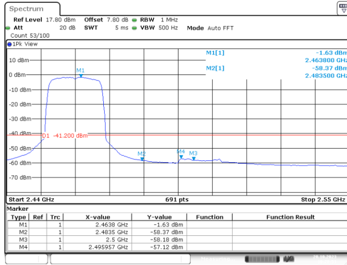
11G_Ant1_High_2462_Peak
