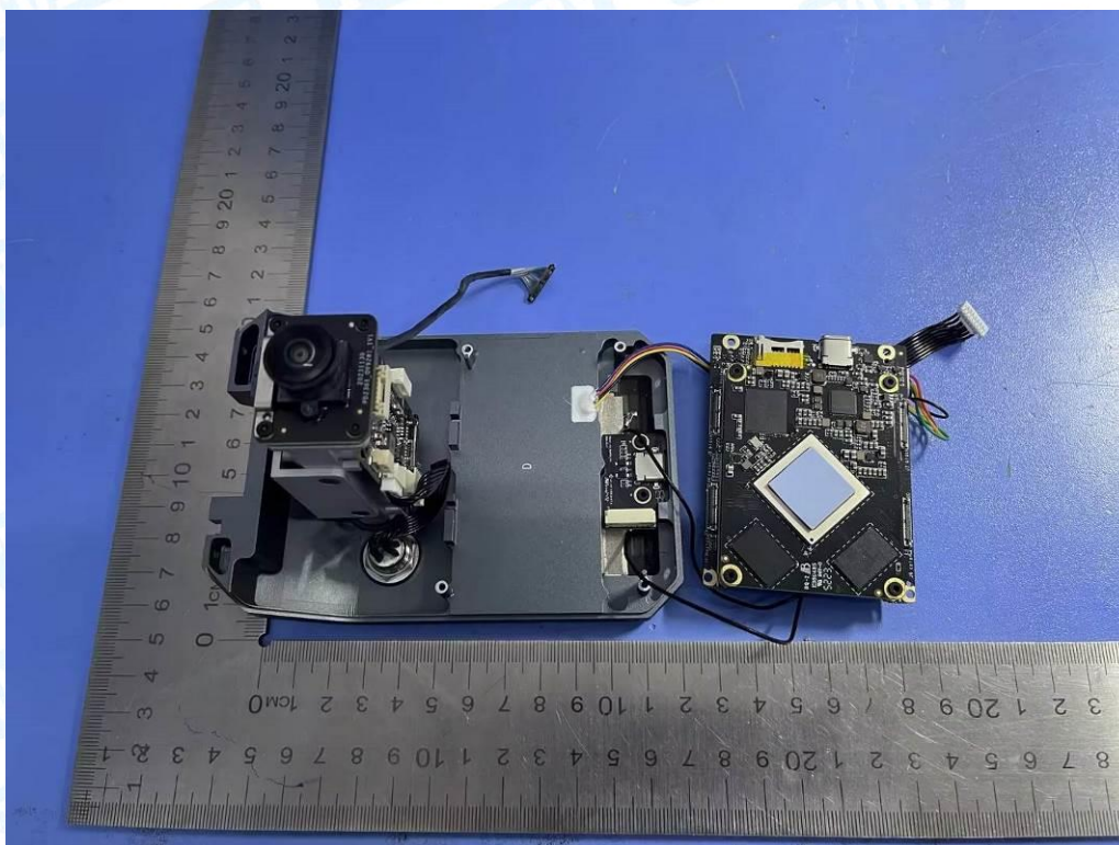
Photo 10 Internal of EUT
