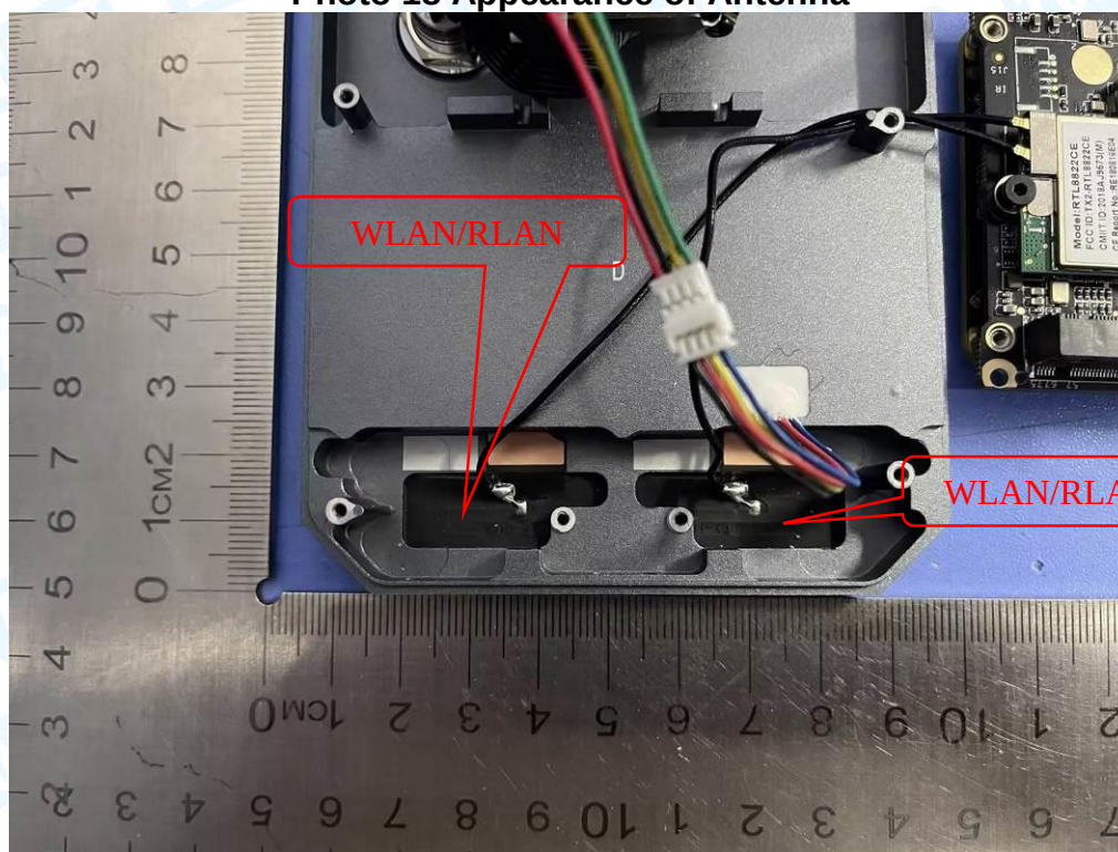
Photo 18 Appearance of Antenna
