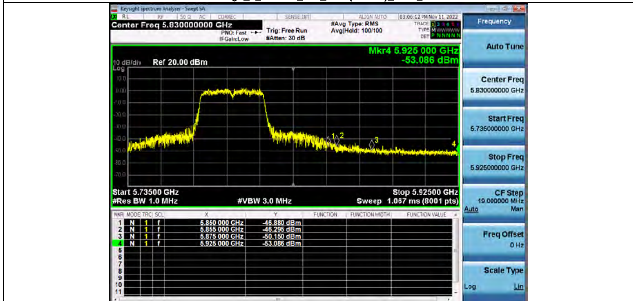
Bandedge 5_8GWiFi_802_11ac(VHT40)_5795_40M
