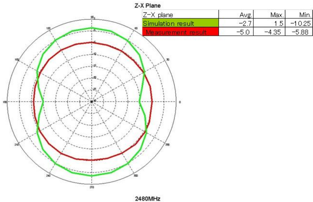
Radiation pattern @2.480GHz
