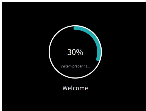
Figure 3.1 Startup View
