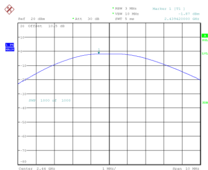
2440 MHz
