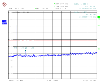
Low Channel
