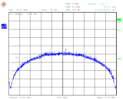
Middle Channel
