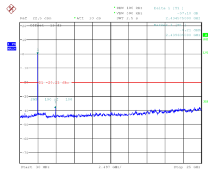
Middle Channel
