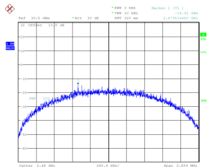
High Channel
