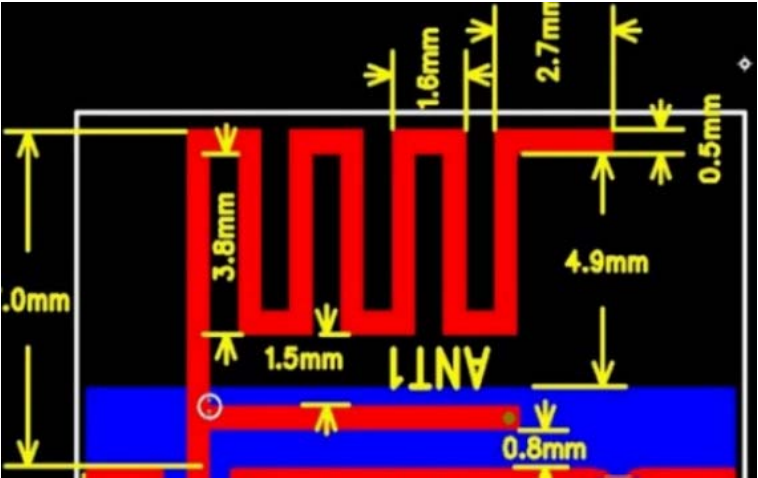
WIFI antenna
