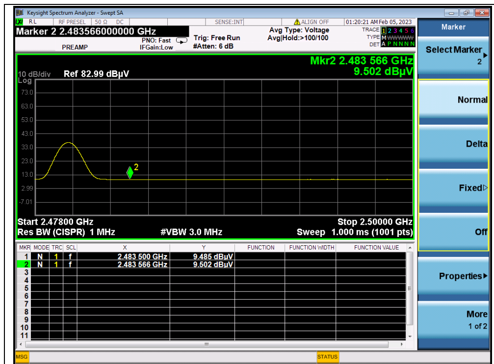
(AVERAGE, Channel 6)
