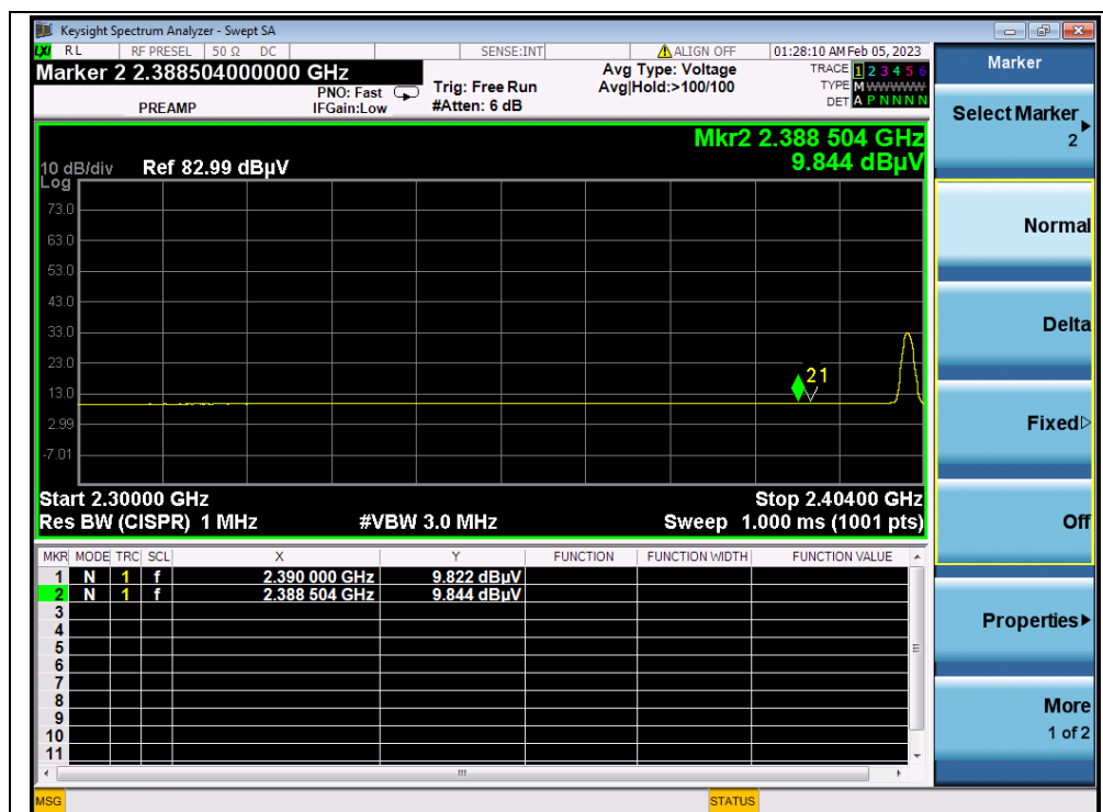
(AVERAGE, Channel 1)
