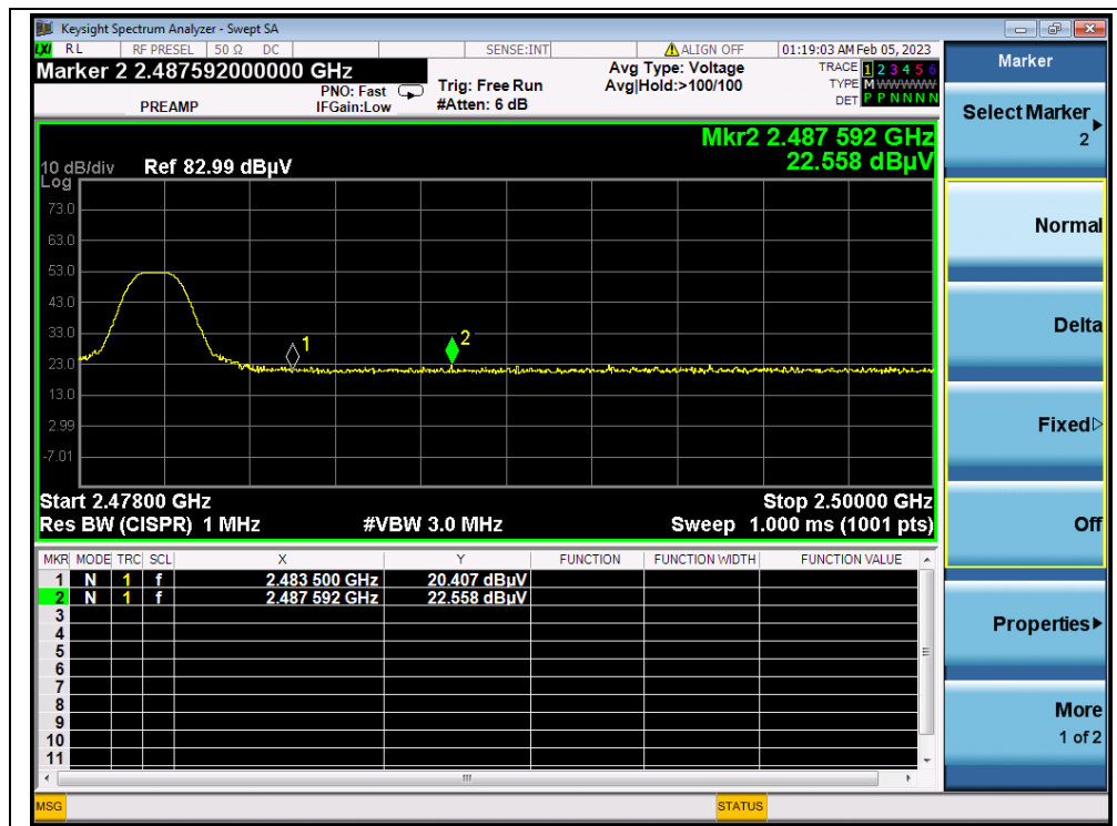
(PEAK, Channel 6)
