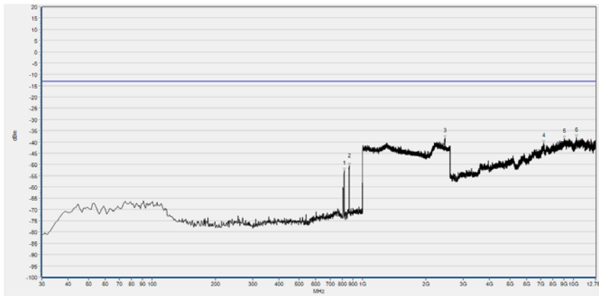
LTE Band 18, 5MHz BW, Low Channel, QPSK
