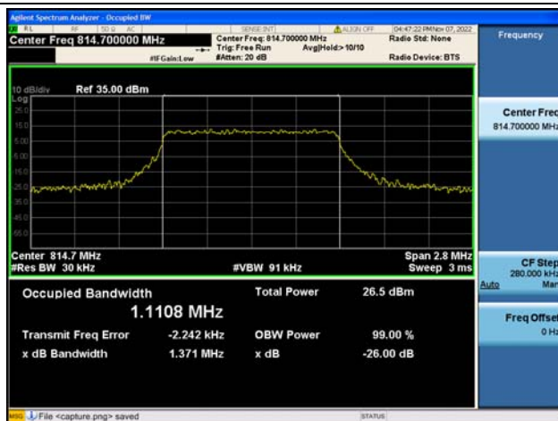
Band26Part90 / 1.4MHz / 16QAM/ Low CH
