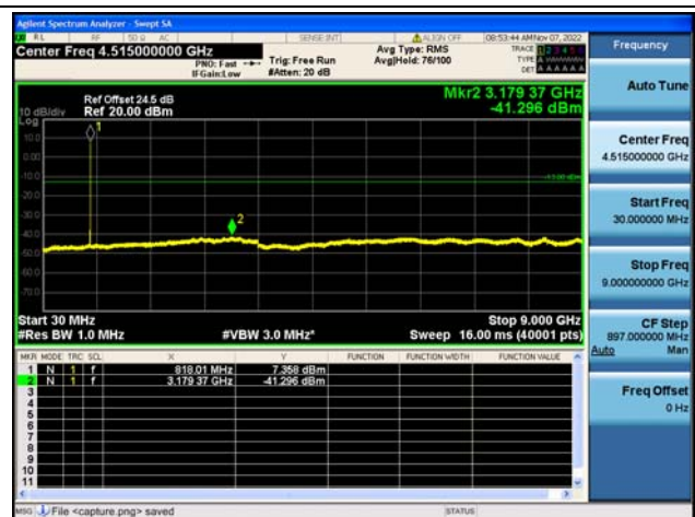
Band26Part90 / 3MHz / Mid CH / 64QAM
