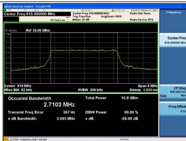
Band26Part90 / 3MHz / 16QAM/ Mid CH
