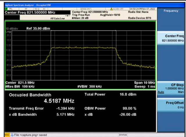
Band26Part90 / 5MHz / QPSK/ High CH
