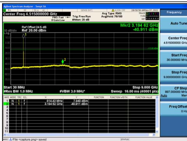
Band26Part90 / 1.4MHz / Low CH / 16QAM
