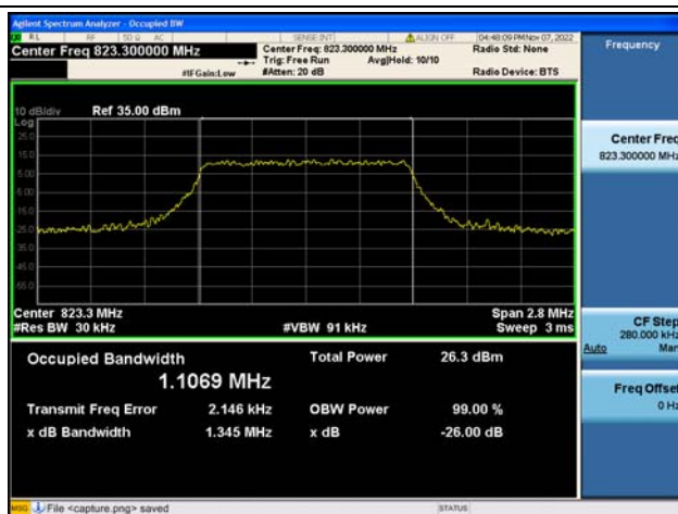
Band26Part90 / 1.4MHz / 16QAM/ High CH
