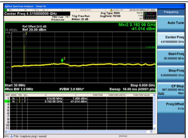
Band26Part90 / 10MHz / Mid CH / 16QAM
