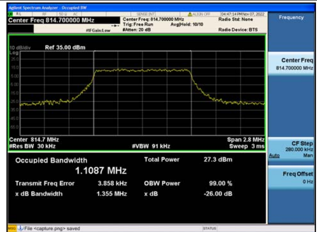
Band26Part90 / 1.4MHz / QPSK/ Low CH
