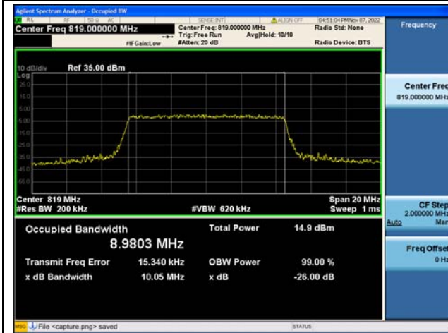
Band26Part90 / 10MHz / 64QAM/ Mid CH
