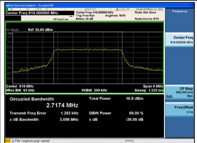
Band26Part90 / 3MHz / QPSK/ Mid CH
