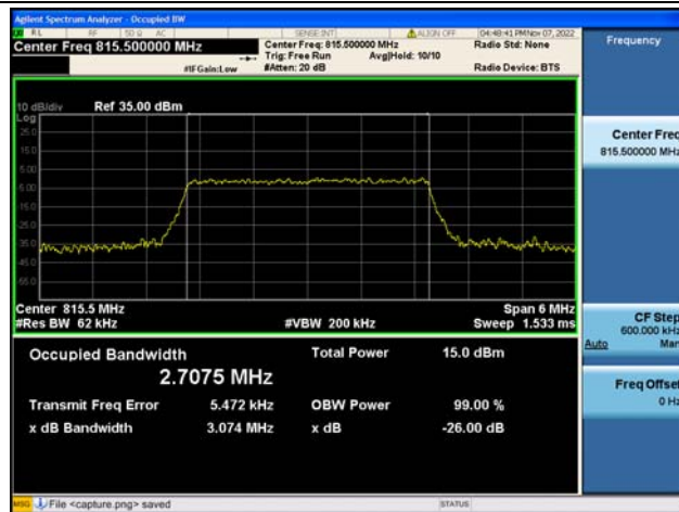
Band26Part90 / 3MHz / 64QAM/ Low CH
