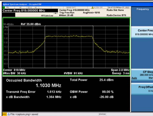
Band26Part90 / 1.4MHz / 64QAM/ Mid CH
