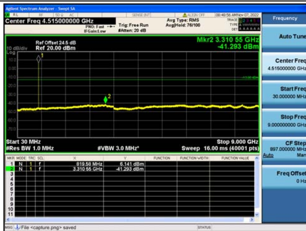
Band18Part90 / 5MHz / High CH / 64QAM
