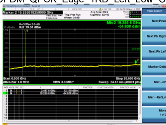
n41(40M)_DFT-s-OFDM_QPSK_Edge_1RB_Left_Low_CH
