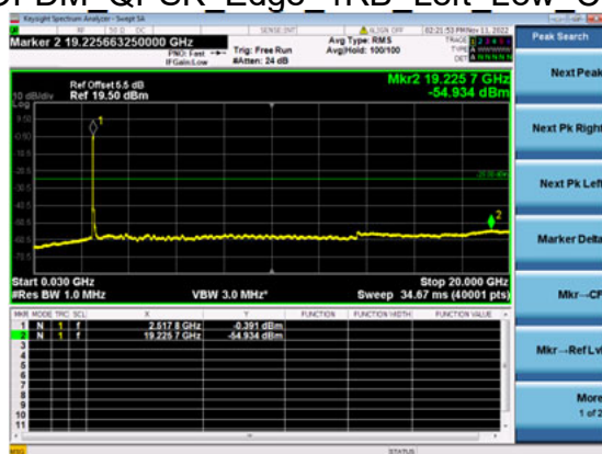
n41(50M)_DFT-s- OFDM_QPSK_Edge_1RB_Left_Low_CH
