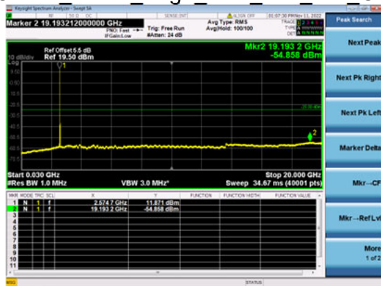
n41(40M)_DFT-s-OFDM_BPSK_Edge_1RB_Left_Mid_CH
