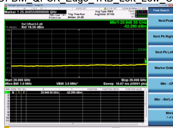
n41(30M)_DFT-s-OFDM_QPSK_Edge_1RB_Left_Low_CH
