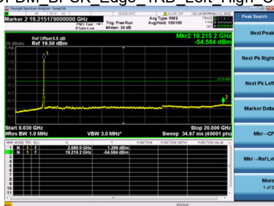
n41(50M)_DFT-s- OFDM_BPSK_Edge_1RB_Left_High_CH
