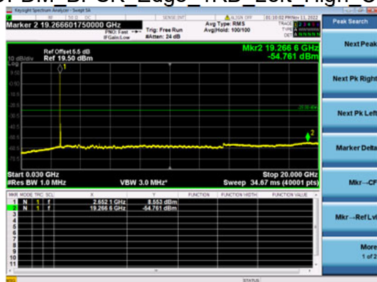
n41(40M)_DFT-s-OFDM_BPSK_Edge_1RB_Left_High_CH
