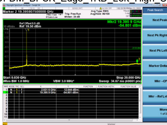
n41(60M)_DFT-s- OFDM_BPSK_Edge_1RB_Left_High_CH
