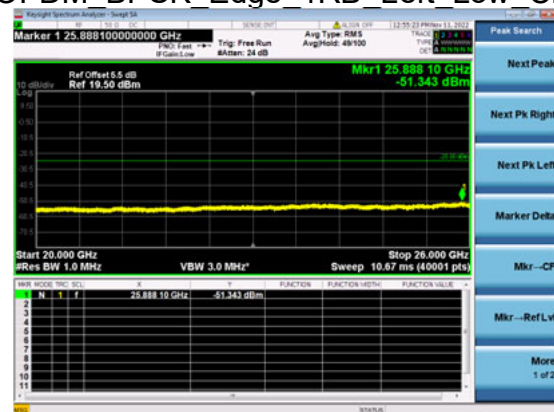
n41(30M)_DFT-s-OFDM_BPSK_Edge_1RB_Left_Low_CH
