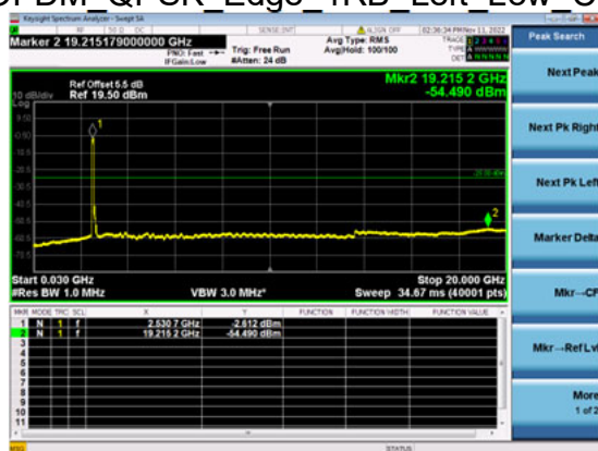
n41(80M)_DFT-s- OFDM_QPSK_Edge_1RB_Left_Low_CH
