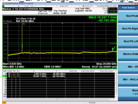
n41(30M)_DFT-s-OFDM_QPSK_Edge_1RB_Left_High_CH
