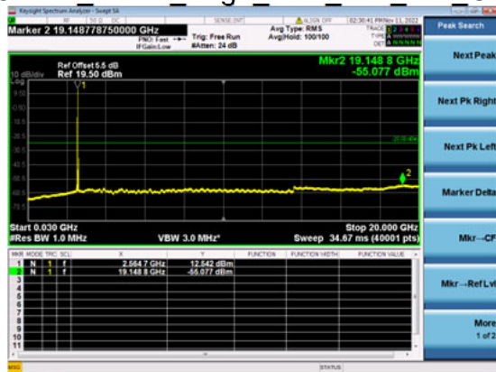
n41(60M)_DFT-s- OFDM_BPSK_Edge_1RB_Left_Mid_CH
