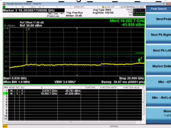
n41(30M)_DFT-s-OFDM_BPSK_Edge_1RB_Left_Mid_CH
