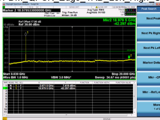
n41(20M)_DFT-s-OFDM_QPSK_Edge_1RB_Left_High_CH
