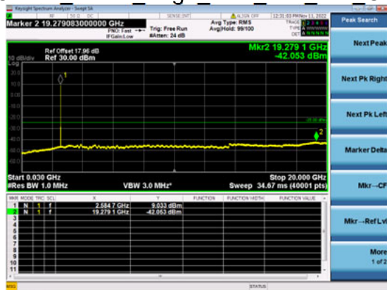
n41(20M)_DFT-s-OFDM_BPSK_Edge_1RB_Left_Mid_CH
