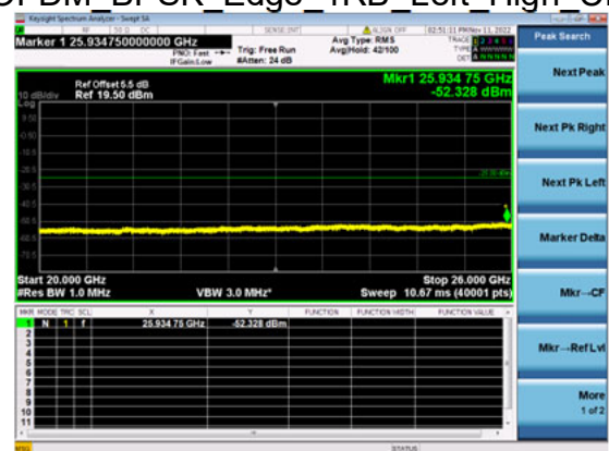
n41(60M)_DFT-s- OFDM_BPSK_Edge_1RB_Left_High_CH
