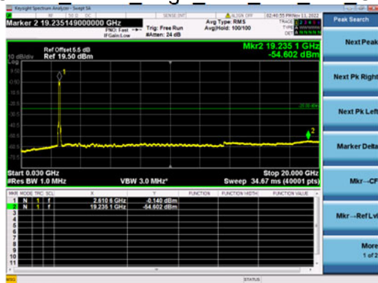
n41(80M)_DFT-s-OFDM_BPSK_Edge_1RB_Left_Mid_CH
