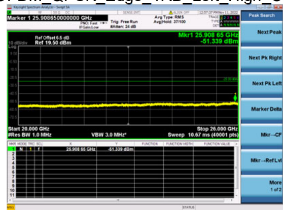
n41(30M)_DFT-s-OFDM_QPSK_Edge_1RB_Left_High_CH
