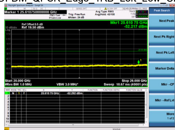
n41(80M)_DFT-s- OFDM_QPSK_Edge_1RB_Left_Low_CH
