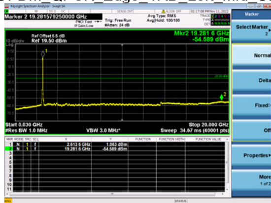
n41(50M)_DFT-s- OFDM_QPSK_Edge_1RB_Left_Mid_CH
