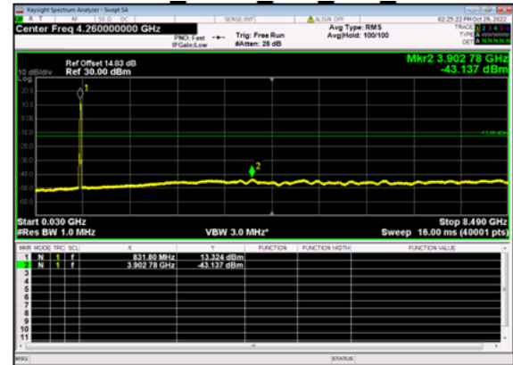
n5(20M)_DFT-s-OFDM_ QPSK Outer Full Mid CH
