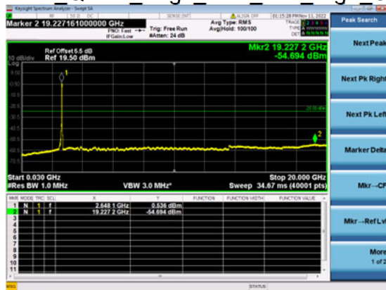
n41(50M)_DFT-s-OFDM_QPSK_Edge_1RB_Left_High_CH
