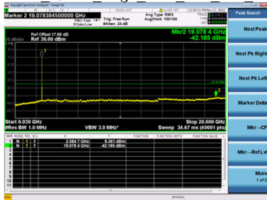
n41(20M)_DFT-s-OFDM_QPSK_Edge_1RB_Left_Mid_CH
