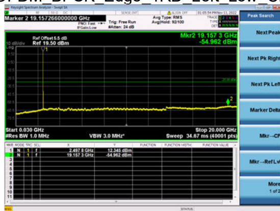
n41(40M)_DFT-s-OFDM_BPSK_Edge_1RB_Left_Low_CH
