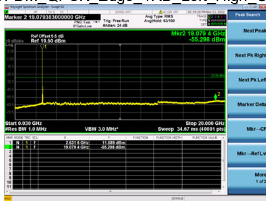
n41(60M)_DFT-s- OFDM_QPSK_Edge_1RB_Left_High_CH
