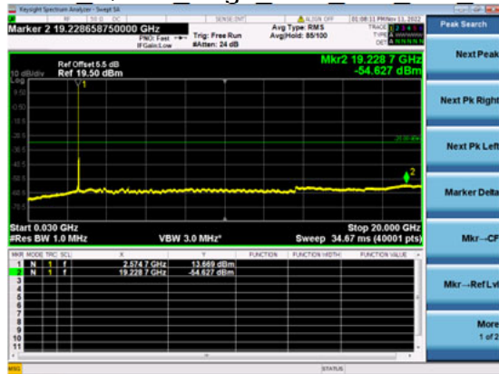
n41(40M)_DFT-s-OFDM_QPSK_Edge_1RB_Left_Mid_CH
