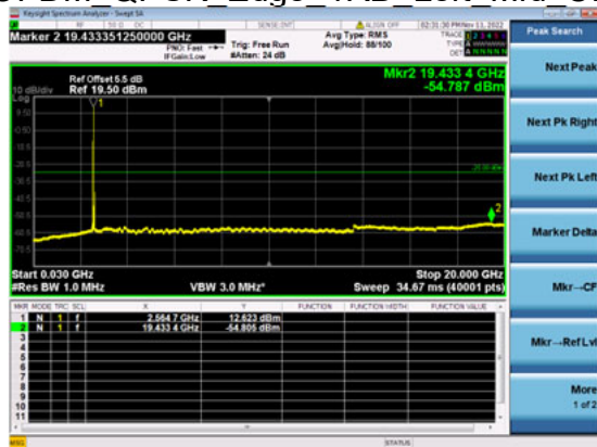
n41(60M)_DFT-s- OFDM_QPSK_Edge_1RB_Left_Mid_CH
