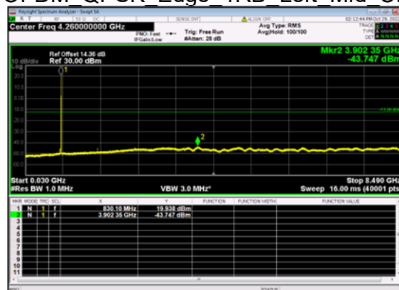
n5(15M)_DFT-s- OFDM QPSK Edge 1RB Left Mid CH
