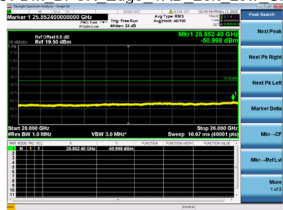
n41(80M)_DFT-s- OFDM_BPSK_Edge_1RB_Left_Low_CH
