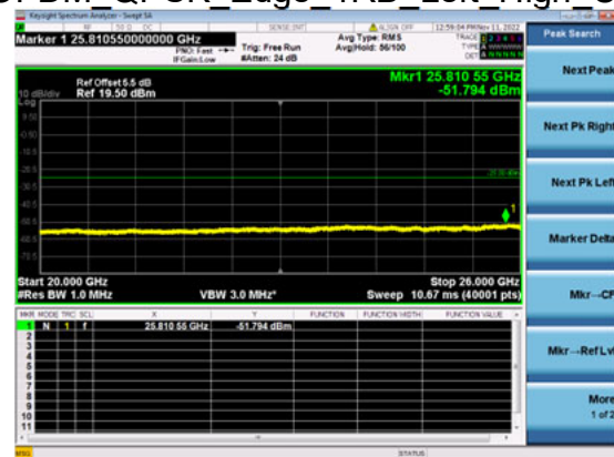
n41(20M)_DFT-s-OFDM_QPSK_Edge_1RB_Left_High_CH
