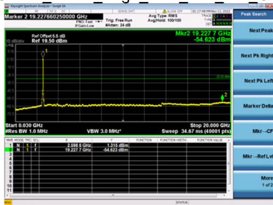
n41(50M)_DFT-s- OFDM_BPSK_Edge_1RB_Left_Mid_CH
