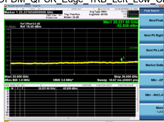
n41(40M)_DFT-s-OFDM_QPSK_Edge_1RB_Left_Low_CH
