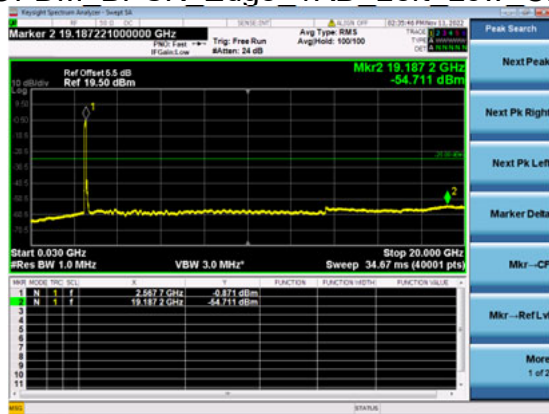
n41(80M)_DFT-s- OFDM_BPSK_Edge_1RB_Left_Low_CH
