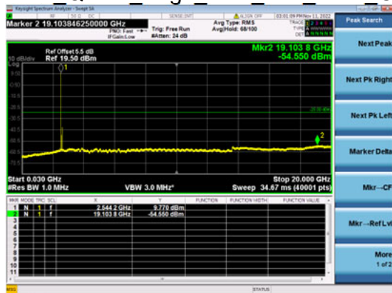
n41(100M)_DFT-s- OFDM_QPSK_Edge_1RB_Left_Mid_CH
