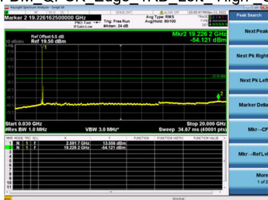
n41(100M)_DFT-s- OFDM_QPSK_Edge_1RB_Left_High_CH
