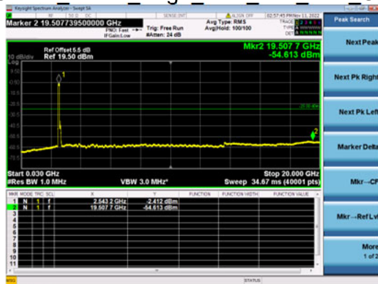
n41(100M)_DFT-s-OFDM_BPSK_Edge_1RB_Left_Low_CH
