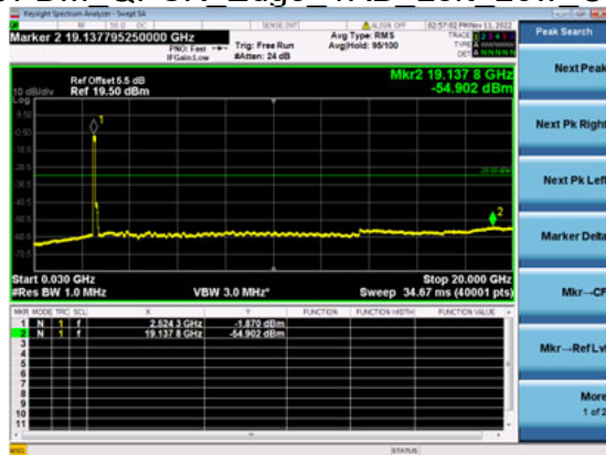
n41(100M)_DFT-s-OFDM_QPSK_Edge_1RB_Left_Low_CH
