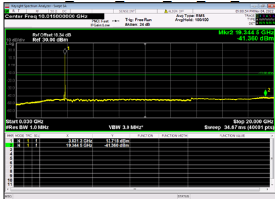
n77(30M)_DFT-s-OFDM BPSK Outer Full Mid CH
