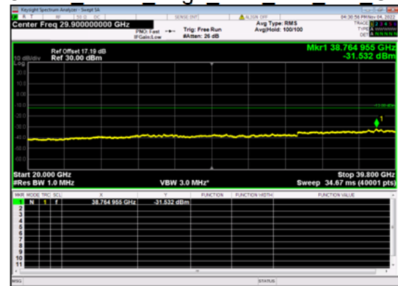
n77(20M)_DFT-s- OFDM BPSK Edge 1RB Left Mid CH
