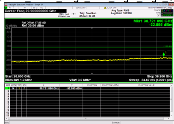
n77(30M)_DFT-s-OFDM BPSK Edge 1RB Right High CH
