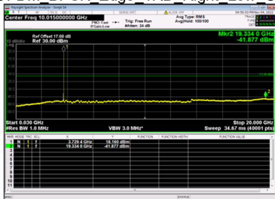
n77(30M)_DFT-s-OFDM BPSK Edge 1RB Right Low CH
