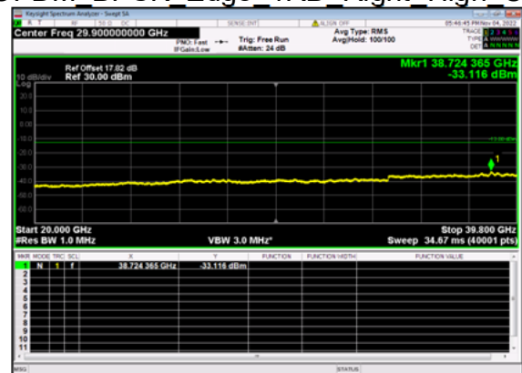
n77(40M)_DFT-s-OFDM BPSK Edge 1RB Right High CH
