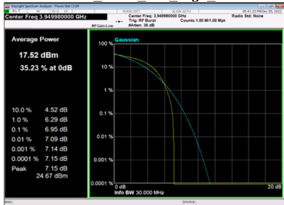
n77(30M)_DFT-s-OFDM_PI_2-BPSK_Outer_Full_High_CH
