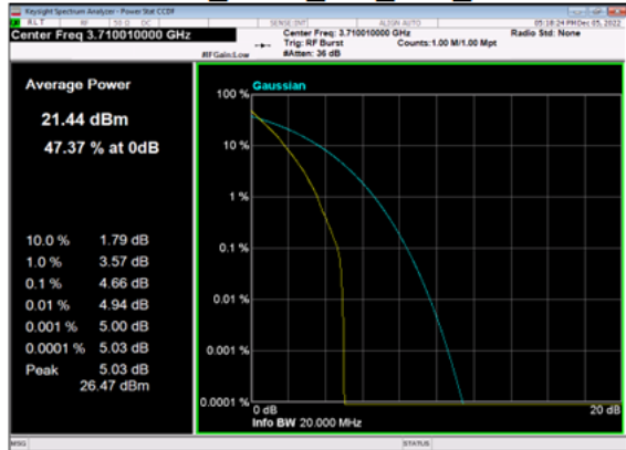
n77(20M)_DFT-s-OFDM_PI_2-BPSK Outer_Full_Low_CH
