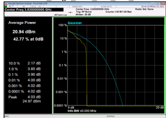
n77(40M)_DFT-s-OFDM_PI_2-BPSK_Edge_1RB_Left Mid_CH
