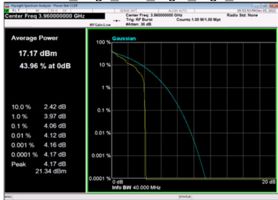
n77(40M)_DFT-s-OFDM_PI_2-BPSK_Edge_1RB_Right_High_CH
