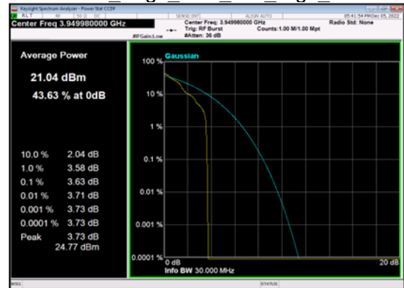
n77(30M)_DFT-s-OFDM_PI_2-BPSK_Edge_1RB_Left_High_CH
