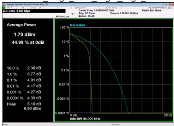
n77(80M)_DFT-s-OFDM_PI_2-BPSK_Edge_1RB_Right_High_CH
