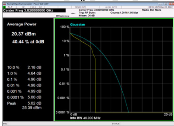
n77(40M)_DFT-s-OFDM_QPSK_Edge_1RB_Left Mid_CH
