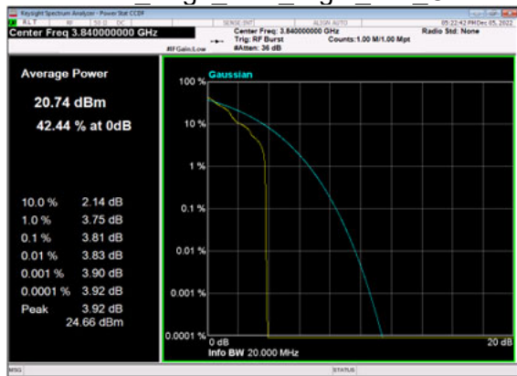
n77(20M)_DFT-s-OFDM_PI_2-BPSK_Edge_1RB_Right Mid_CH
