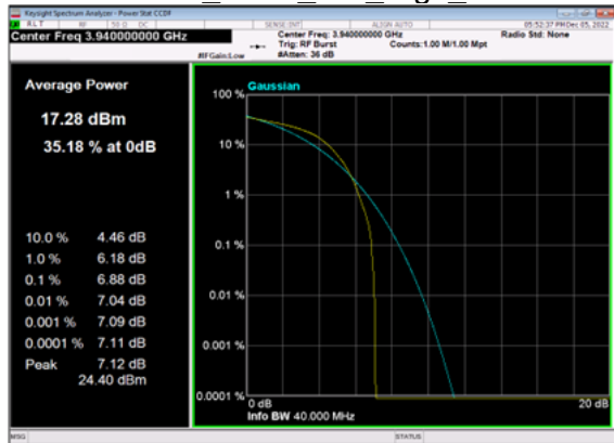
n77(40M)_DFT-s-OFDM_PI_2-BPSK_Outer_Full_High_CH
