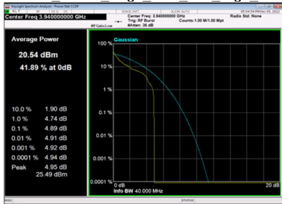
n77(40M)_DFT-s-OFDM_QPSK_Edge_1RB_Left_High_CH
