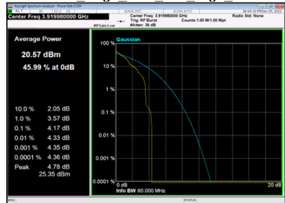
n77(60M)_DFT-s-OFDM_PI_2-BPSK_Edge_1RB_Left_High_CH
