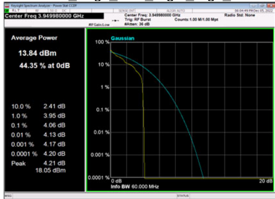
n77(60M)_DFT-s-OFDM_PI_2-BPSK_Edge_1RB_Right_High_CH
