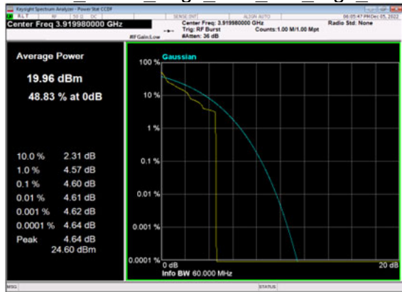
n77(60M)_DFT-s-OFDM_QPSK_Edge_1RB_Left_High_CH
