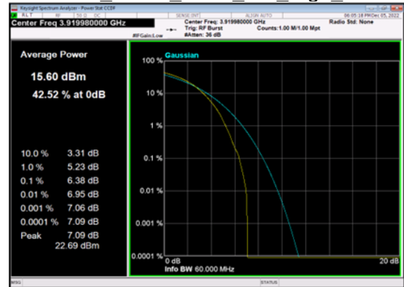
n77(60M)_DFT-s-OFDM_QPSK_Outer_Full_High_CH
