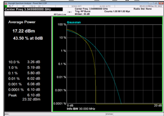
n77(30M)_DFT-s-OFDM_QPSK_Outer_Full_High_CH
