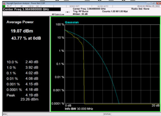
n77(30M)_DFT-s-OFDM_PI_2-BPSK_Edge_1RB_Right_High_CH
