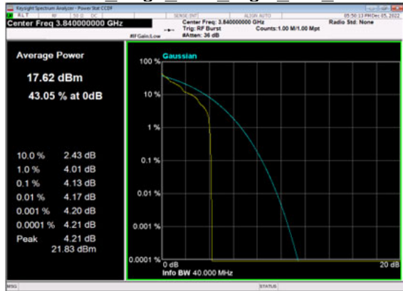
n77(40M)_DFT-s-OFDM_PI_2-BPSK_Edge_1RB_Right Mid_CH
