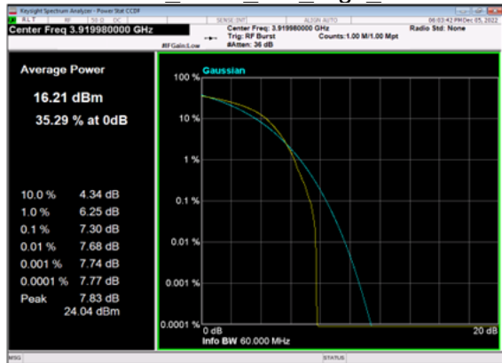
n77(60M)_DFT-s-OFDM_PI_2-BPSK_Outer_Full_High_CH
