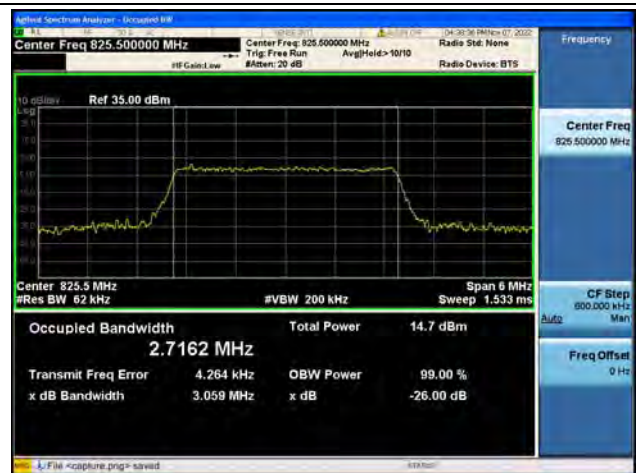
Band26Part22 / 3MHz / 64QAM / Low CH
