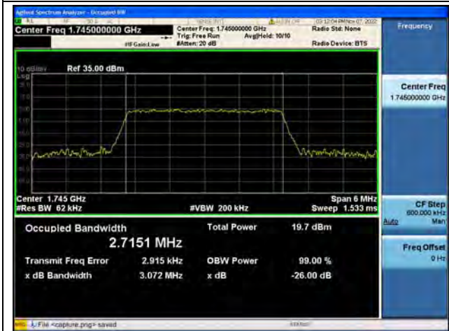
Band66 / 3MHz / 64QAM/ Mid CH
