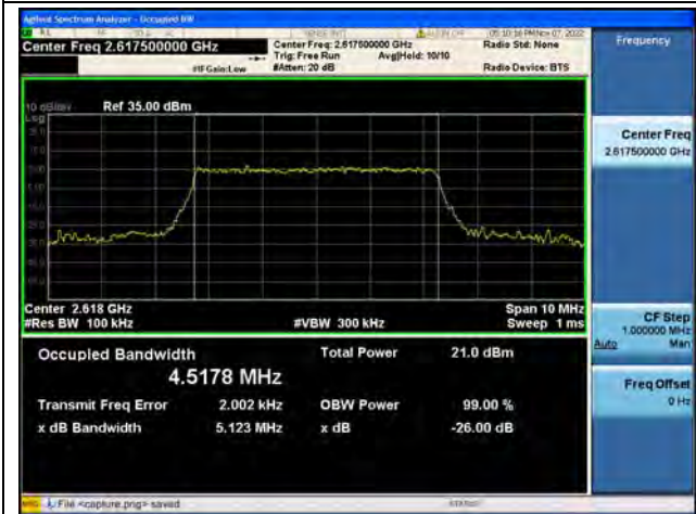
Band38 / 5MHz / 64QAM/ High CH
