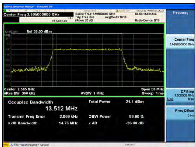
Band38 / 15MHz / 64QAM/ Mid CH
