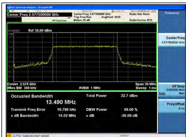
Band38 / 15MHz / QPSK/ Low CH
