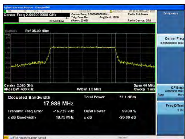
Band38 / 20MHz / 16QAM/ Mid CH
