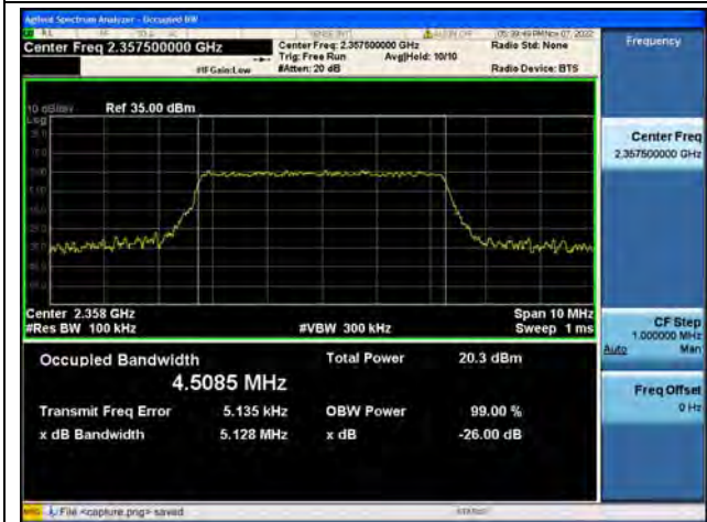
Band40-2 / 5MHz / 64QAM/ High CH
