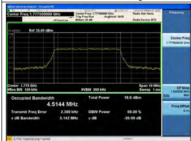
Band66 / 5MHz / 64QAM/ High CH
