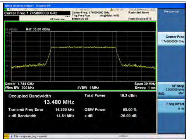
Band66 / 15MHz / 64QAM/ Mid CH
