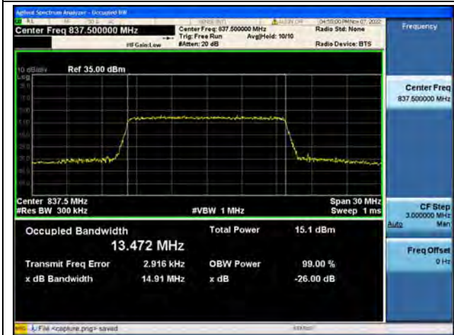
Band19 / 15MHz / 64QAM/ Low CH
