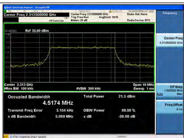
Band40-1 / 5MHz / 16QAM/ High CH
