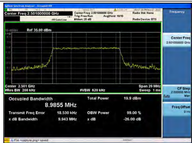
Band41 / 10MHz / 64QAM/ Low CH
