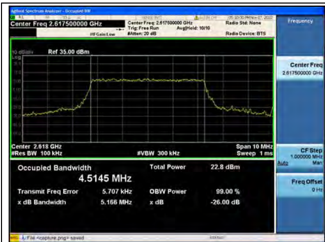
Band38 / 5MHz / QPSK/ High CH
