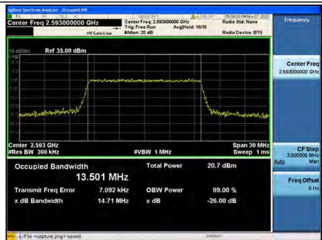
Band41 / 15MHz / 64QAM/ Mid CH
