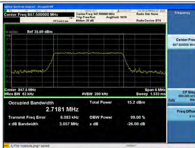
Band26Part22 / 3MHz / 64QAM/ High CH
