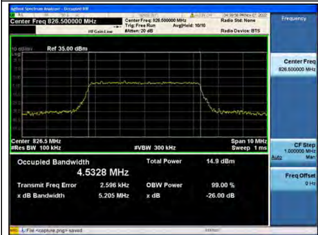
Band26Part22 / 5MHz / 64QAM/ Low CH
