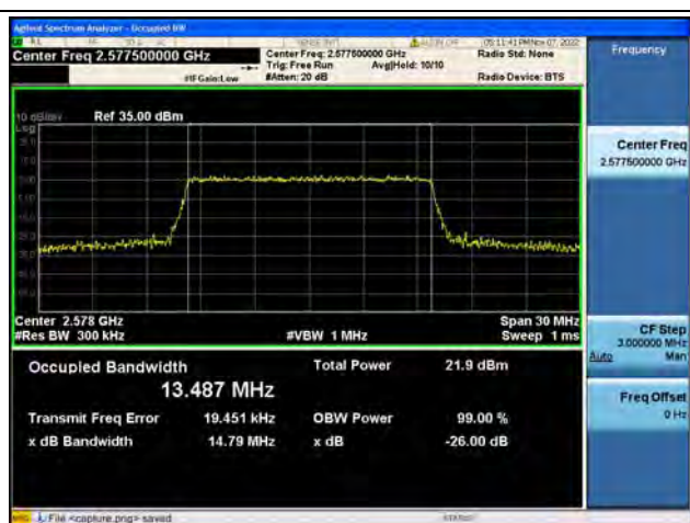
Band38 / 15MHz / 16QAM/ Low CH
