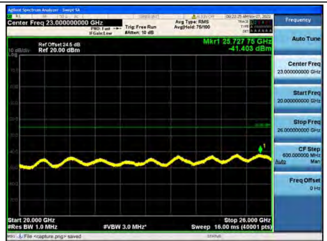
Band7-20G-26G / 5MHz / Mid CH / 64QAM
