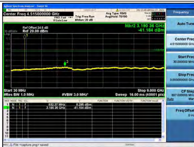
Band26Part22 / 10MHz / Mid CH / 16QAM
