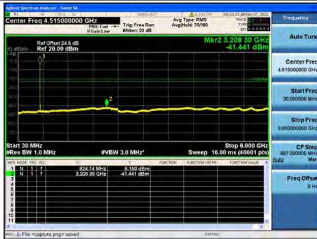
Band26Part22 / 10MHz / Low CH / 64QAM
