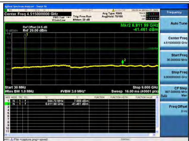
Band26Part22 / 5MHz / High CH / 64QAM
