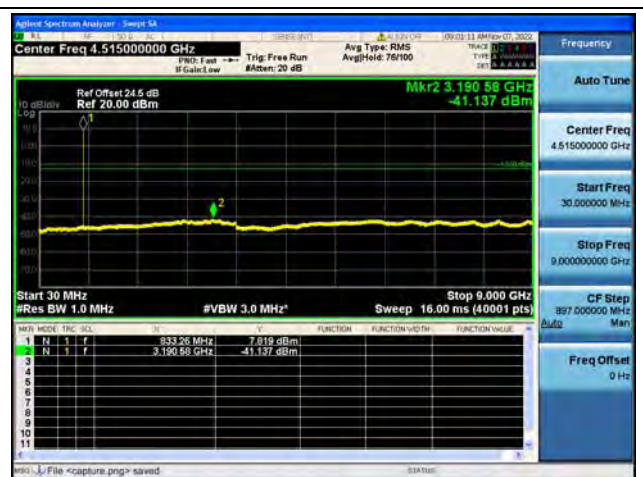
Band19 / 10MHz / Mid CH / 16QAM
