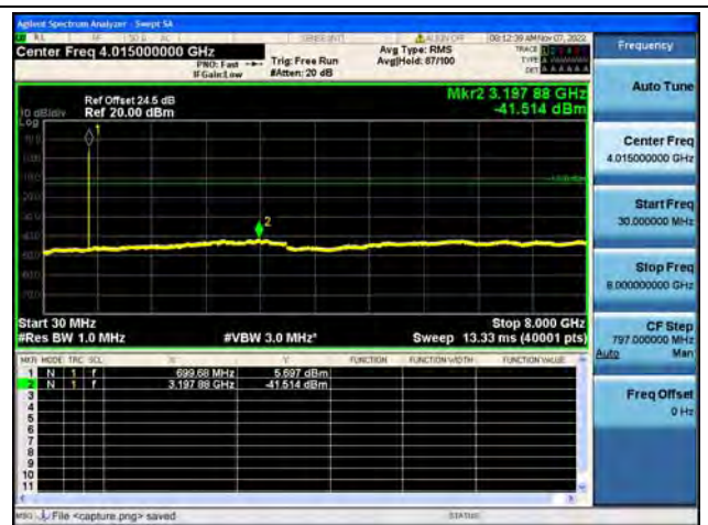
Band12 / 5MHz / Low CH / 16QAM
