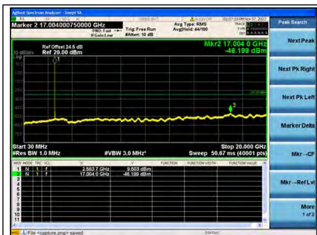
Band41-30M-20G / 20MHz / Mid CH / QPSK
