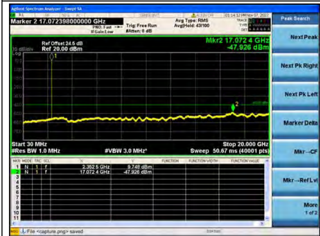
Band40-2-30M-20G / 5MHz / Mid CH / 16QAM
