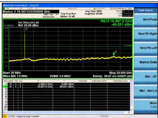
Band41-30M-20G / 10MHz / Mid CH / 64QAM
