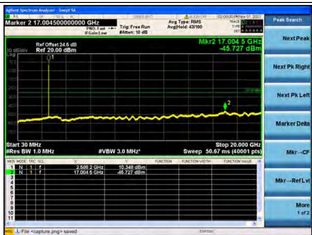
Band41-30M-20G / 10MHz / Mid CH / 16QAM
