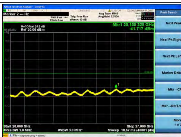
Band41-20G-27G / 20MHz / Mid CH / 64QAM
