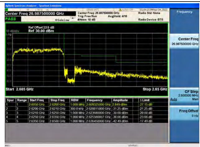
Band38 / 15MHz / High CH / QPSK / FULL RB
