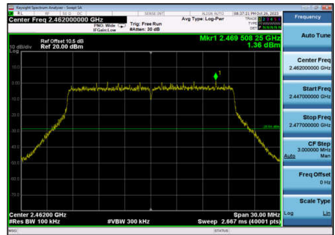
,Plot 1,Reference Level-802.11ax(HE20 ,2462MHz,Ant6
