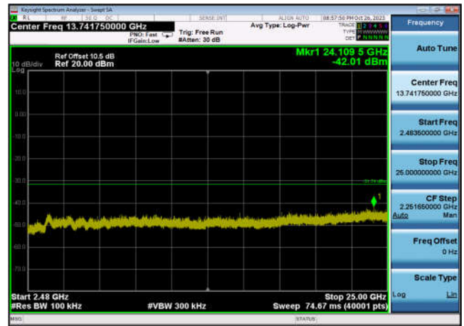
,Plot 4,2483.5MHz~25000MHz-802.11ax(HE40), 2437MHz,Ant6
