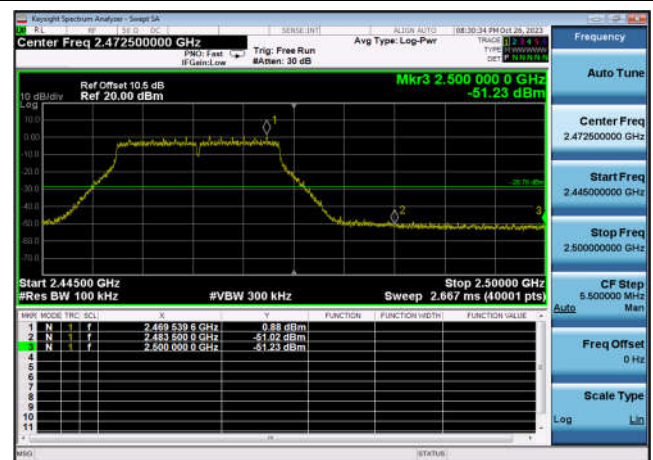
,Plot 2,Band Edge-802.11n(HT20) ,2462MHz,Ant6
