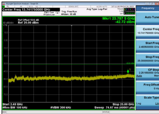
,Plot 4,2483.5MHz~25000MHz-802.11ax(E40), 2452MHz,Ant7
