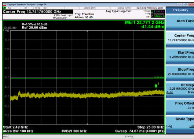
,Plot 4,2483.5MHz~25000MHz-802.11n(HT 40),2452MHz,Ant7
