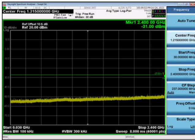
,Plot 3,30MHz~2400MHz-802.11g,2437MHz ,Ant7
