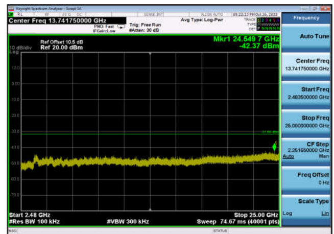
,Plot 4,2483.5MHz~25000MHz-802.11n(HT 40),2452MHz,Ant6
