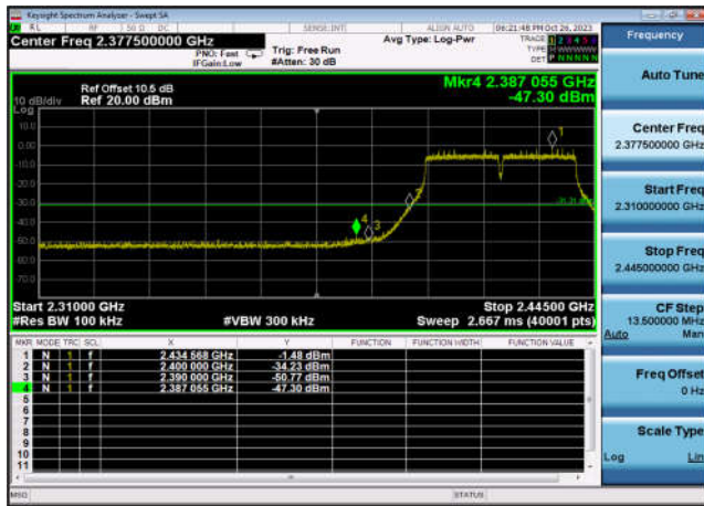
,Plot 2,Band Edge-802.11n(HT40) ,2437MHz,Ant7
