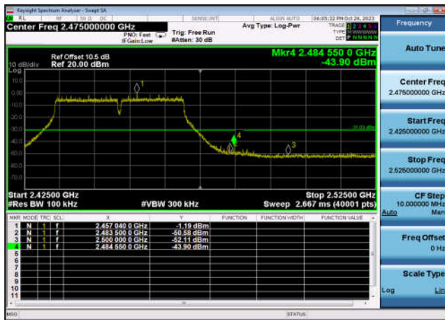
,Plot 2,Band Edge-802.11n(HT40) ,2452MHz,Ant7
