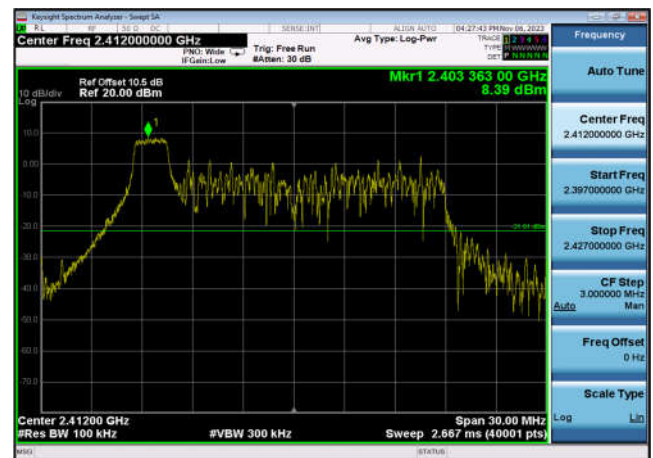
,Plot 1,Reference Level-802.11ax(HE20 _RU26_1),2412MHz,Ant7
