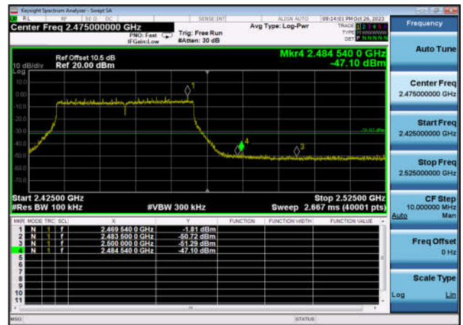
,Plot 2,Band Edge-802.11ax(HE40) ,2452MHz,Ant6
