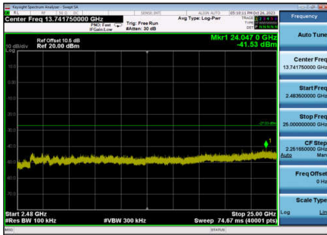
,Plot 4,2483.5MHz~25000MHz-802.11g ,2437MHz,Ant7
