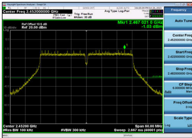
,Plot 1,Reference Level-802.11n(HT40) ,2452MHz,Ant7
