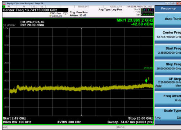
,Plot 4,2483.5MHz~25000MHz-802.11g ,2462MHz,Ant7
