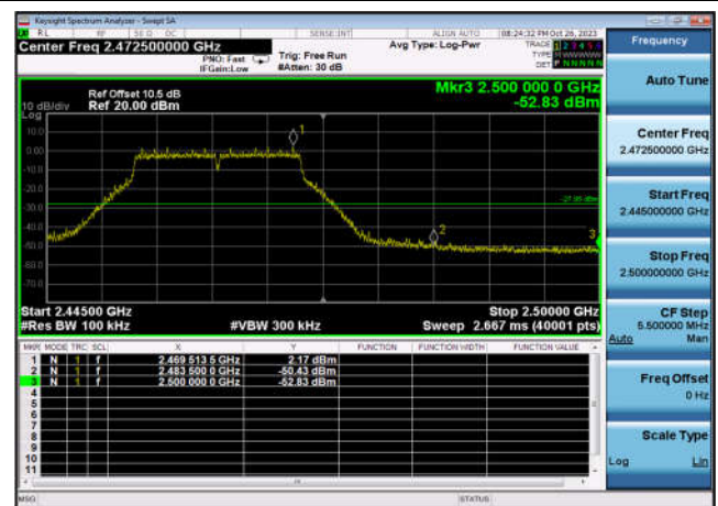
,Plot 2,Band Edge-802.11g,2462MHz ,Ant6
