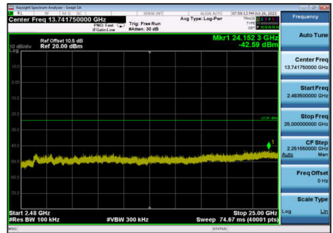
,Plot 4,2483.5MHz~25000MHz-802.11b ,2462MHz,Ant6
