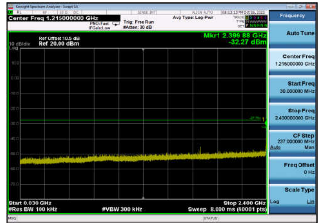
,Plot 3,30MHz~2400MHz-802.11g,2437MHz ,Ant6
