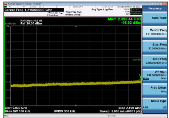
,Plot 3,30MHz~2400MHz-802.11b,2462MHz ,Ant6
