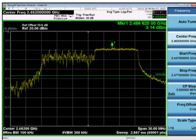
,Plot 1,Reference Level-802.11ax(HE20 _RU106_2),2462MHz,Ant6
