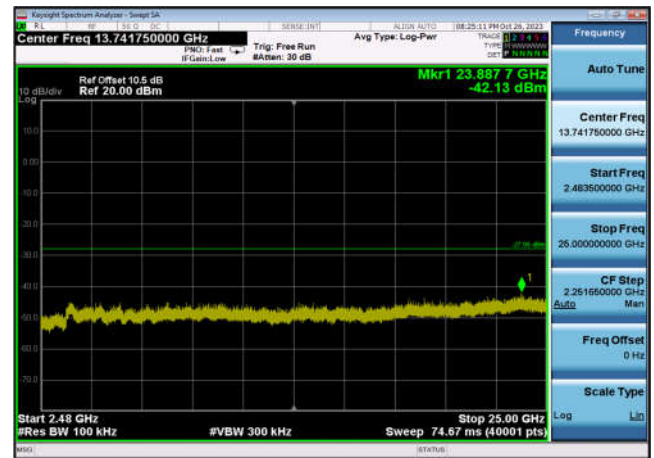
,Plot 4,2483.5MHz~25000MHz-802.11g ,2462MHz,Ant6
