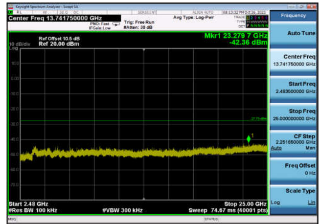
,Plot 4,2483.5MHz~25000MHz-802.11g ,2437MHz,Ant6
