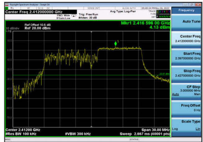
,Plot 1,Reference Level-802.11ax(HE20 _RU106_2),2412MHz,Ant7
