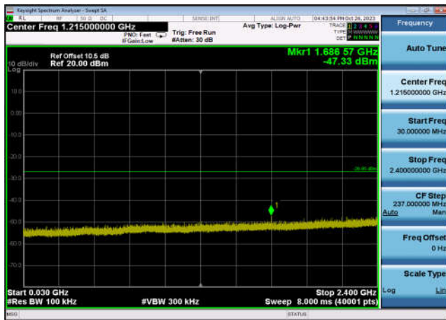
,Plot 3,30MHz~2400MHz-802.11g,2462MHz ,Ant7
