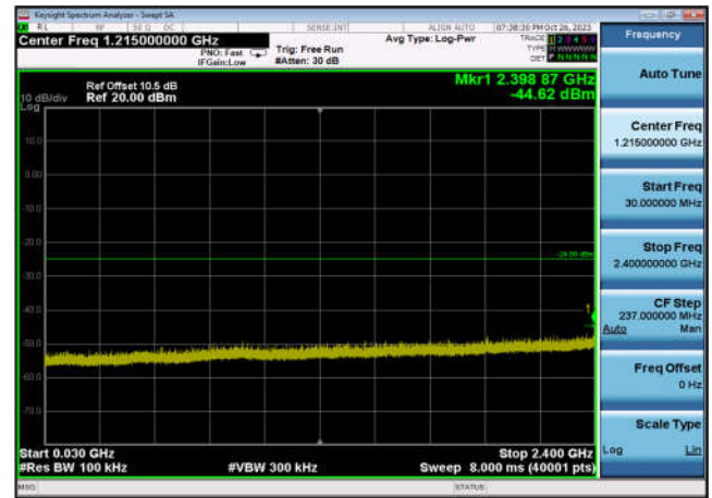
,Plot 3,30MHz~2400MHz-802.11b,2437MHz ,Ant6
