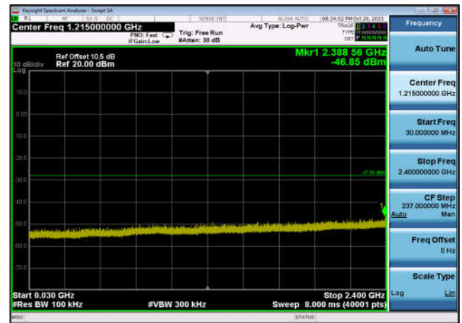
,Plot 3,30MHz~2400MHz-802.11g,2462MHz ,Ant6
