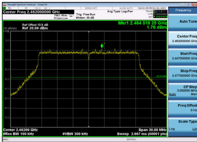
,Plot 1,Reference Level-802.11ax(HE20 ,2462MHz,Ant7
