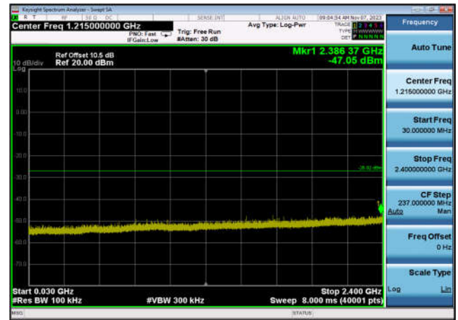
,Plot 3,30MHz~2400MHz-802.11ax(HE20 _RU106_2),2412MHz,Ant7
