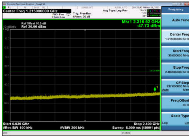
,Plot 3,30MHz~2400MHz-802.11ax(HE20 _RU106_1),2462MHz,Ant7
