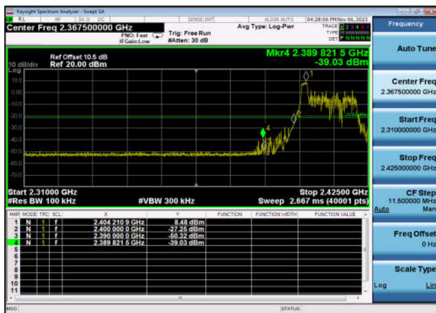
,Plot 2,Band Edge-802.11ax(HE20 _RU26_1),2412MHz,Ant7
