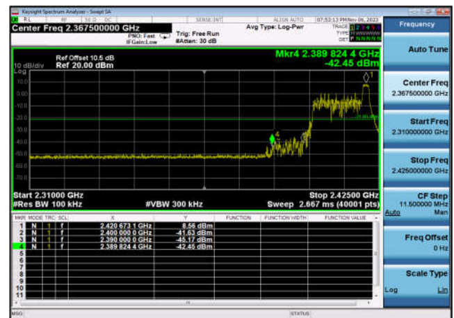
,Plot 2,Band Edge-802.11ax(HE20 _RU26_9),2412MHz,Ant6
