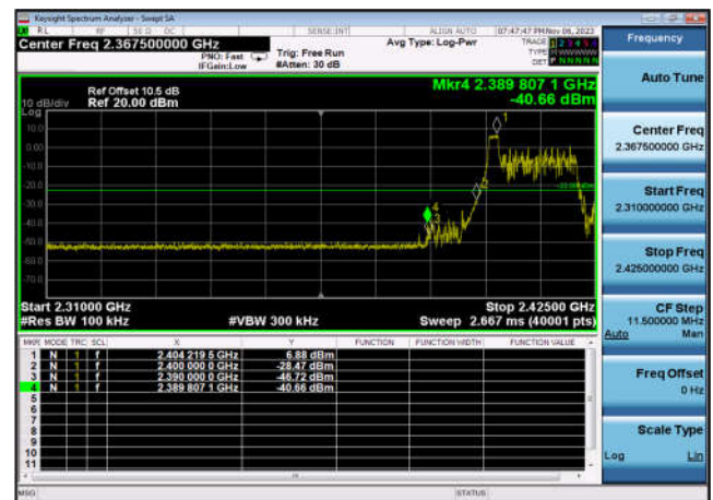
,Plot 2,Band Edge-802.11ax(HE20 _RU26_1),2412MHz,Ant6
