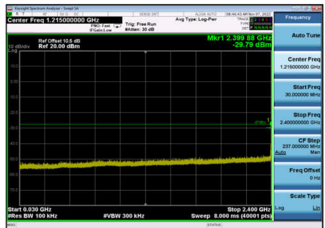
,Plot 3,30MHz~2400MHz-802.11ax(HE20 _RU106_1),2412MHz,Ant6
