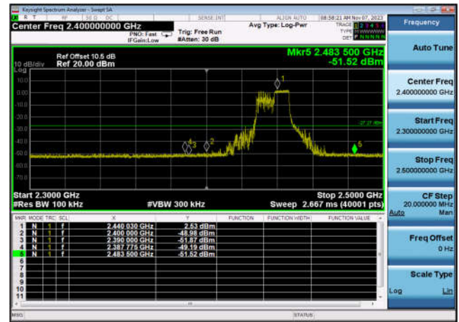
,Plot 2,Band Edge-802.11ax(HE20 _RU106_2),2462MHz,Ant6
