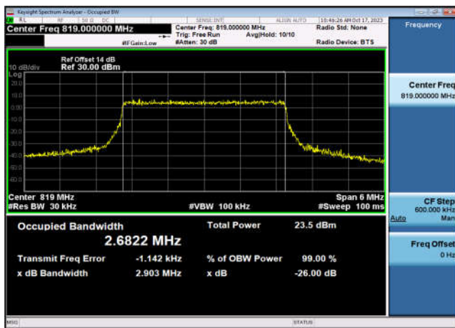
FDD26_Part 90_MidRange_5_819_Q16
