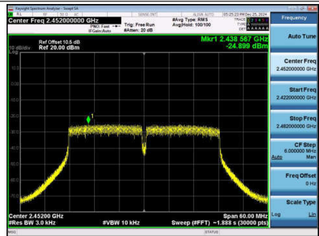
11N40MIMO-Ant2-2452-PASS
