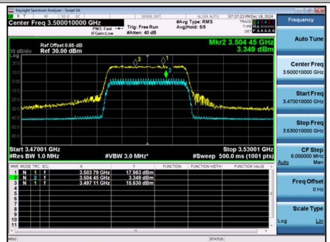
NTNT-n77(3450-3550)-PC2-30-20-M-CP-256QAM-Outer_Full-Ant1-PASS
