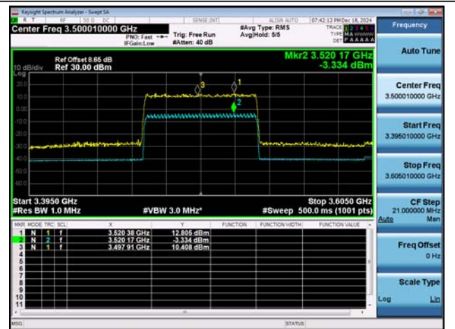
NTNT-n77(3450-3550)-PC2-30-70-M-CP-256QAM-Outer_Full-Ant1-PASS
