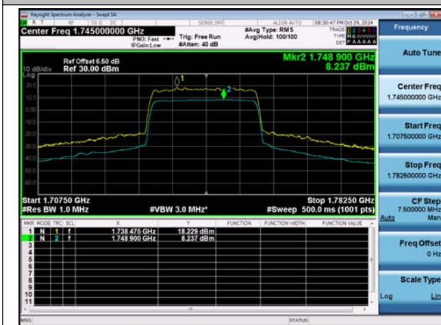
NTNT-n66-PC3-15-25-M-DFT-256QAM-Outer_Full-Ant1-PA
