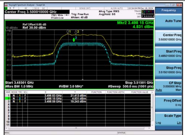
NTNT-n77(3450-3550)-PC2-30-10-M-CP-256QAM-Outer_Full-Ant1-PASS
