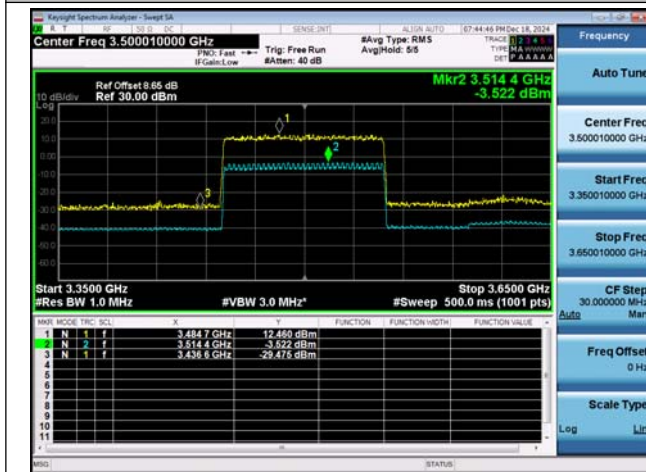
NTNT-n77(3450-3550)-PC2-30-100-M-DFT-256QAM-Out_ Full-Ant1-PASS
