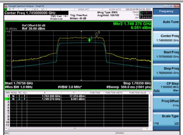
NTNT-n66-PC3-15-25-M-CP-256QAM-Outer_Full-Ant1-PA
