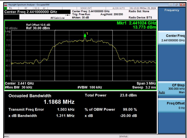
3DH5-Ant2-2441
