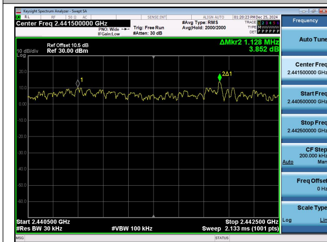
3DH5-Ant2-Hop-PASS
