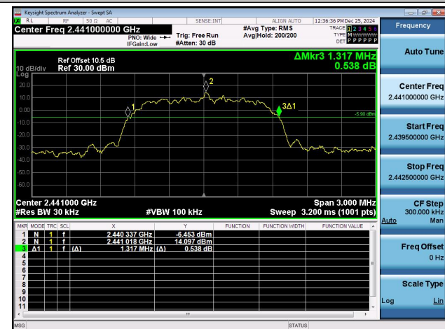
2DH5-Ant2-2441
