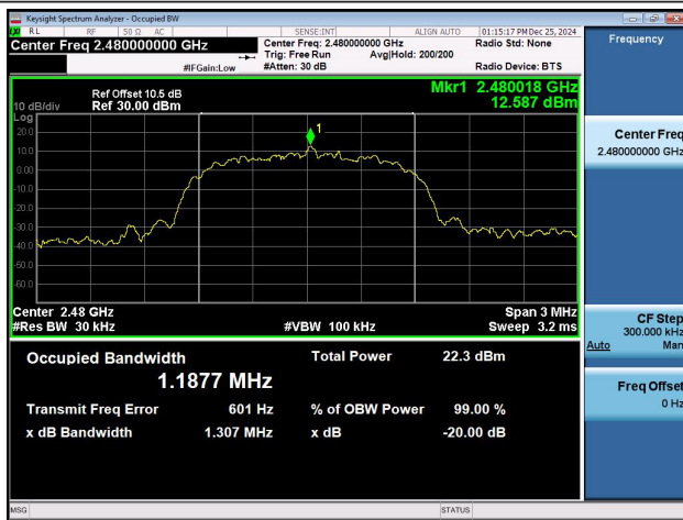
3DH5-Ant2-2480
