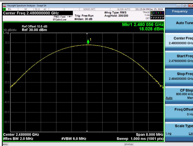
3DH5-Ant2-2480-PASS
