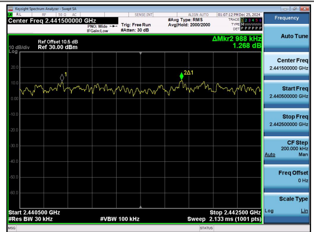
2DH5-Ant2-Hop-PASS
