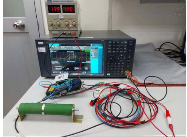
Part 15_209_WPC_Conducted_Setup
