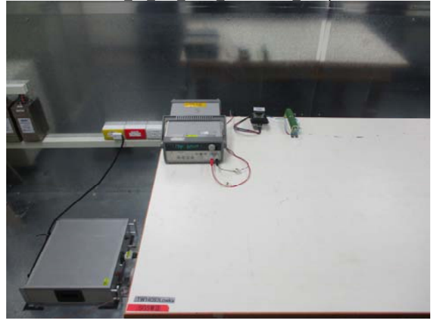
Part 15_209_WPC_Conduction_Setup
