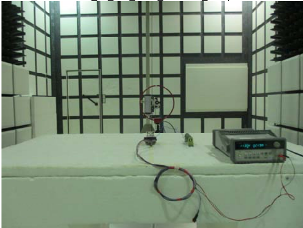
Part 15_209_WPC_Radiated_Setup
