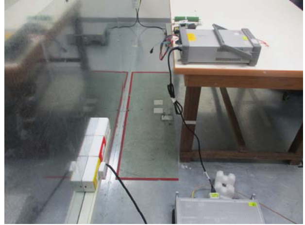
Part 15_209_WPC_Conducted_Setup
