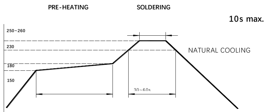
Reflow Soldering
