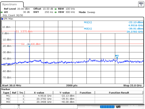
2DH1_High
