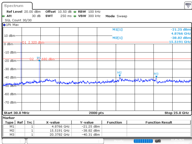
2DH1_Middle
