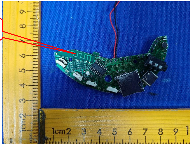
PCB Antenna
