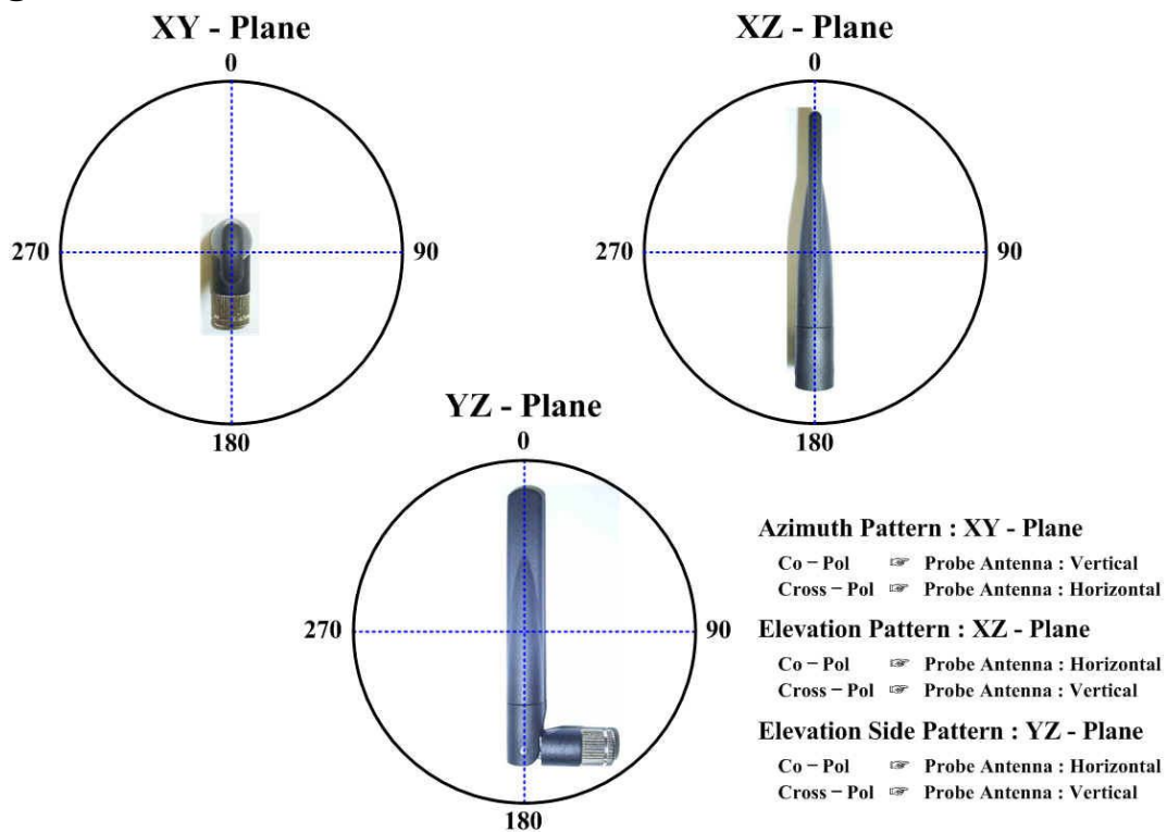
Fig 5. Axis Definitions (Antenna Center)
