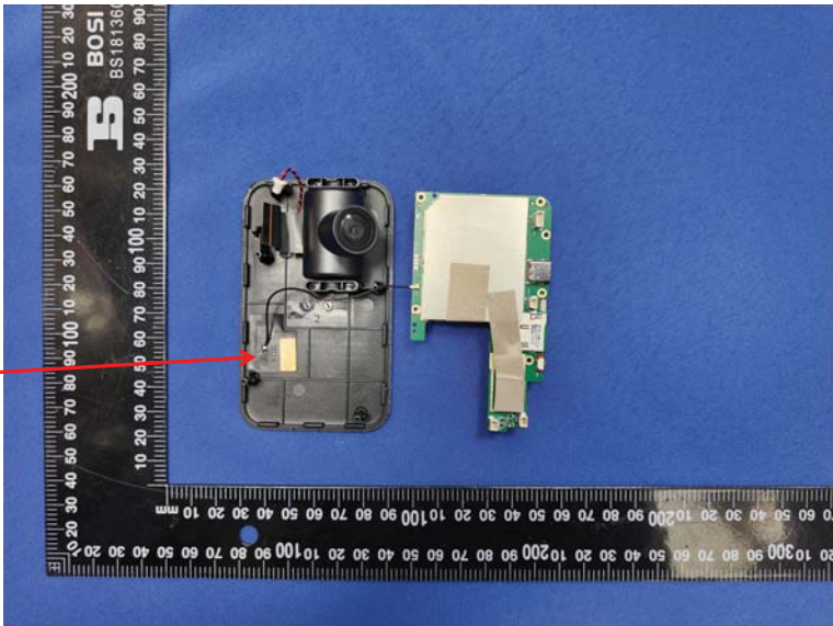
WIFI/Bluetooth Antenna
