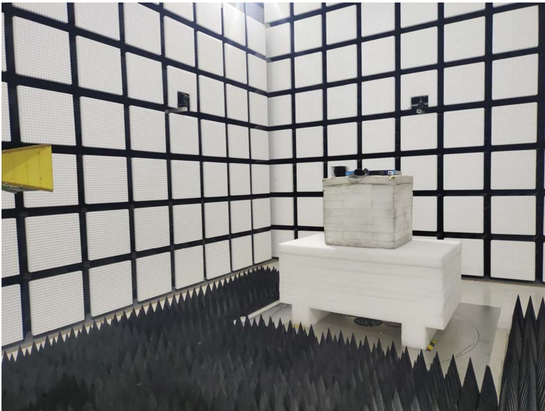
Radiated Emission Above 1GHz View AC
