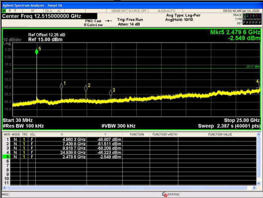
30.0 MHz - 25000.0 MHz GFSK Channel 39
