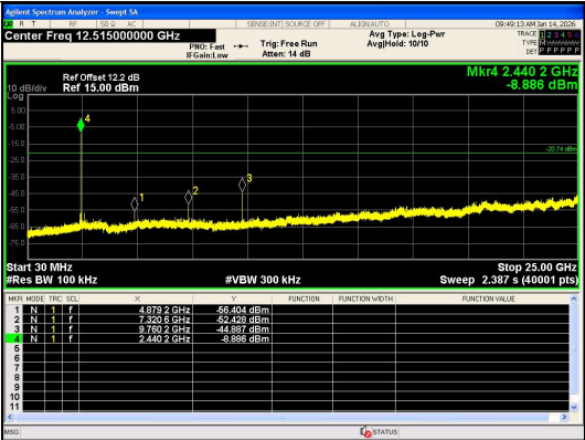
30.0 MHz - 25000.0 MHz GFSK Channel 19
