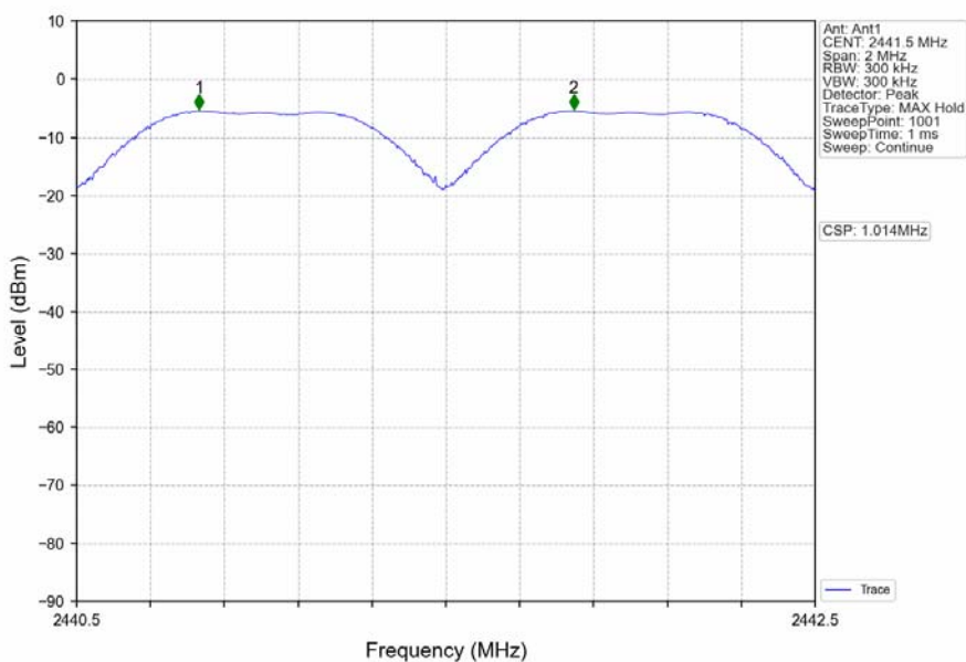
Test plots GFSK Middle Channel
