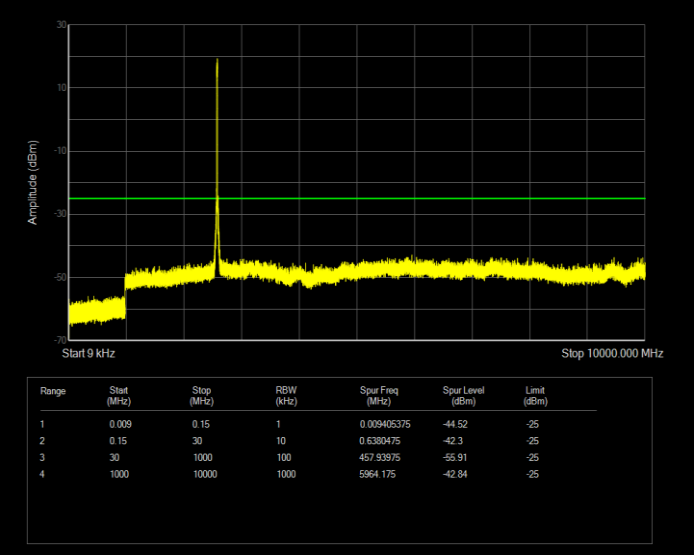
Band41 QAM16 BW=15MHz Channel=40620 RB Size=75 Position=#0
