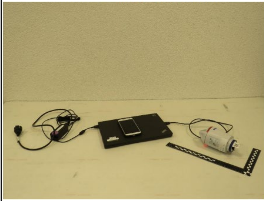
01 TEST SETUP WITH SUPPORT EQUIPMENT
