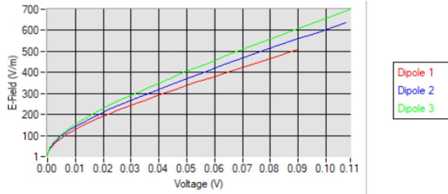
Calibration curves
