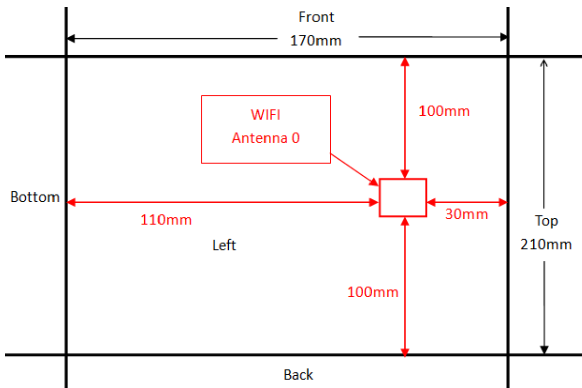
Antenna Configuration 1
