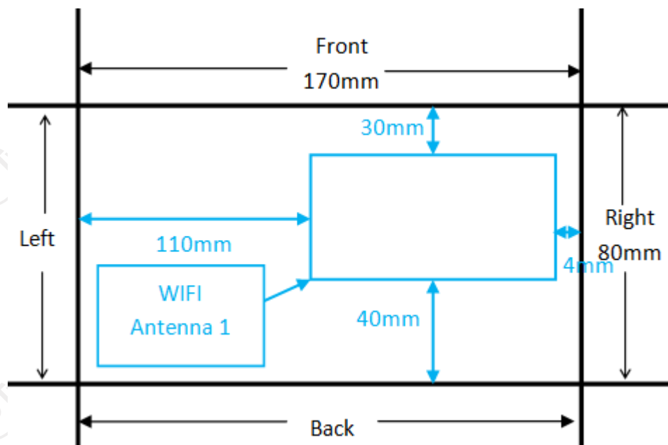
Antenna Configuration 2
