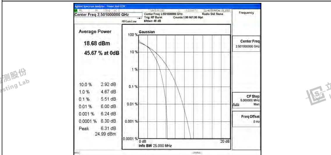
Band41-10MHz-16QAM-40620-50RB#0
