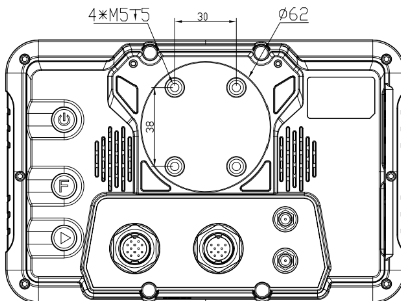
Installation Dimensions
