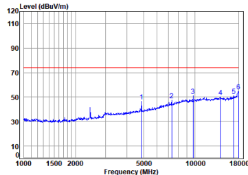
BLE_1M_TX_CH_19_Vertical-Peak
