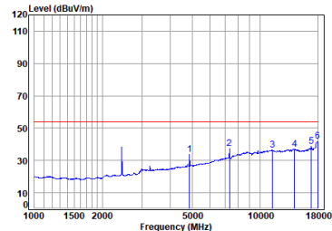
BLE_1M_TX_CH_19_Vertical-Avg
