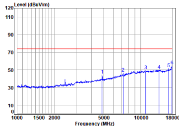
BLE_2M_TX_CH_19_Vertical-Peak
