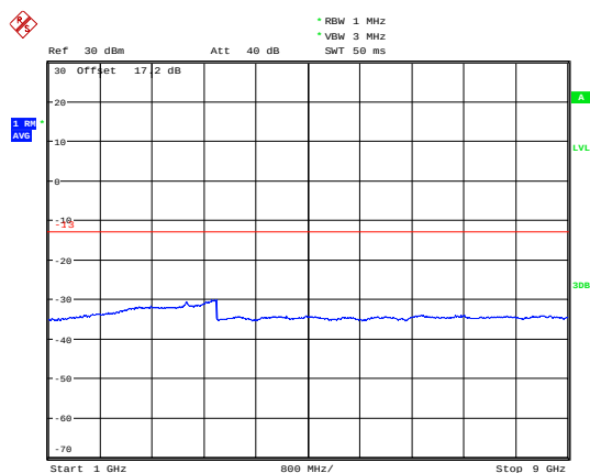
LTE Band 85 10MHz CH-Middle 1GHz~9GHz
