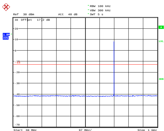
LTE Band 85 10MHz CH- High 30MHz~1GHz
