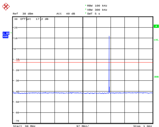
LTE Band 85 10MHz CH- Low 30MHz~1GHz
