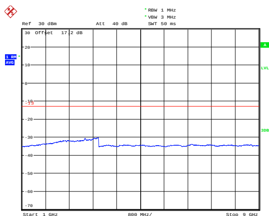
LTE Band 85 10MHz CH- High 1GHz~9GHz
