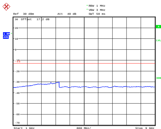
LTE Band 85 10MHz CH- Low 1GHz~9GHz
