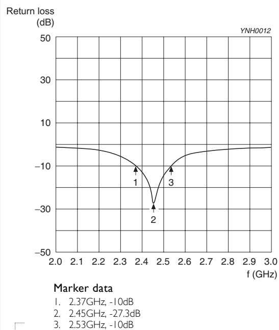
Fig. 4 Return loss
