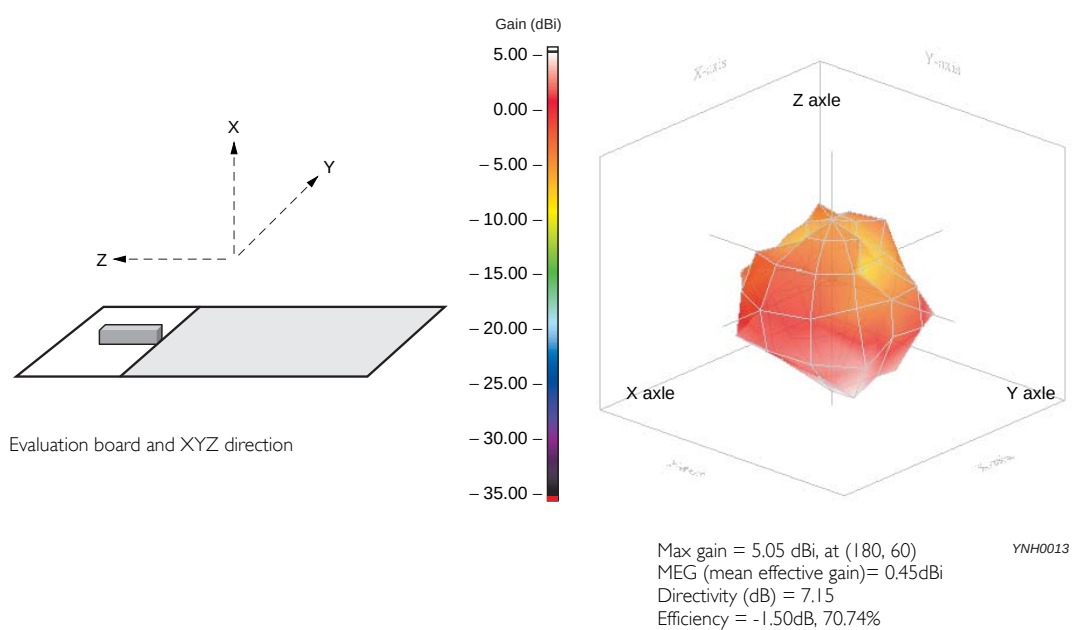
Fig. 5 Radiation pattern
