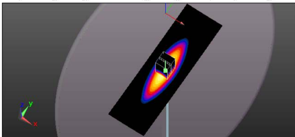
System Performance Check 450MHz Head 250mW
