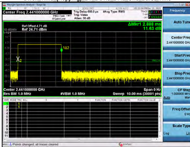
Dwell Time (Hopping) BT_1-DH5_2441_One Burst Time
