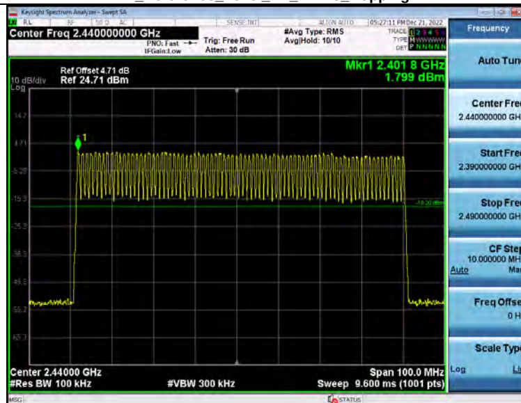
1 Reference Level BT 1-DH5 Hopping
