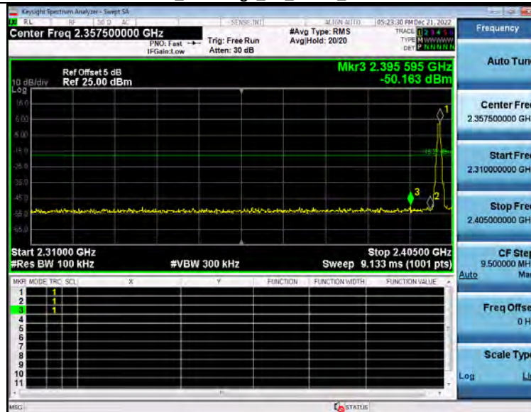
2 Bandedge BT 1-DH5 2402
