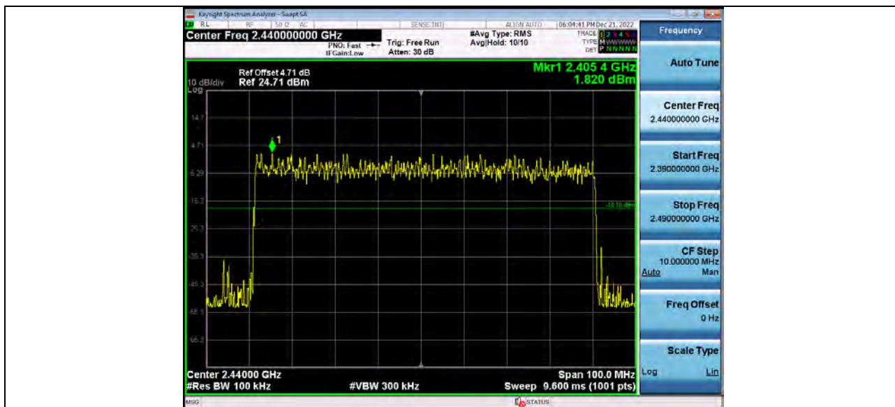
2. Band Edge (Hopping) BT 3-DH5 Hopping
