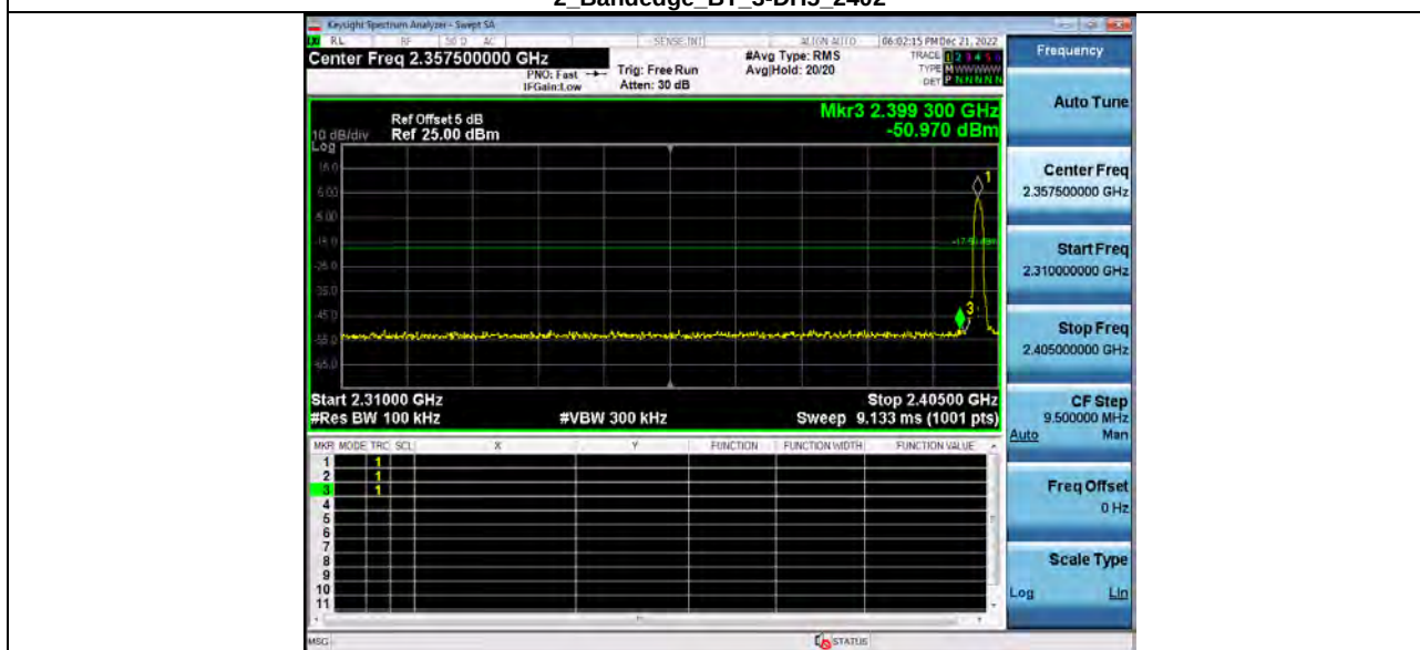
2. Bandedge BT_3-DH5_2402
