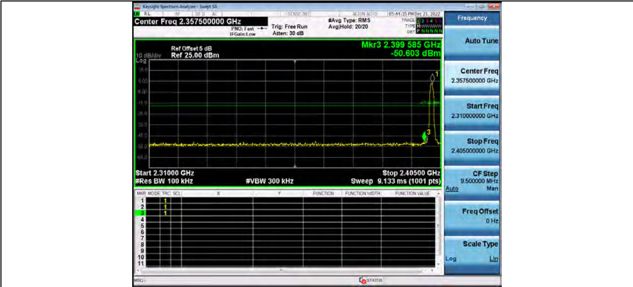
1 Reference_Level_BT_2-DH5_Hopping
