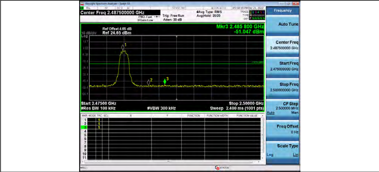
2_Bandedge_BT_2-DH5_2480
