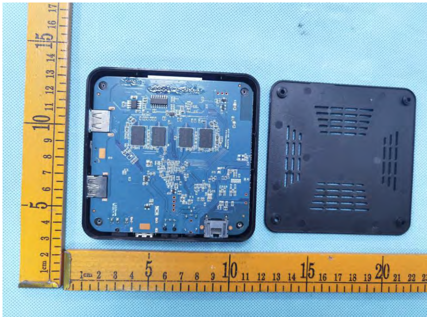
internal photos
