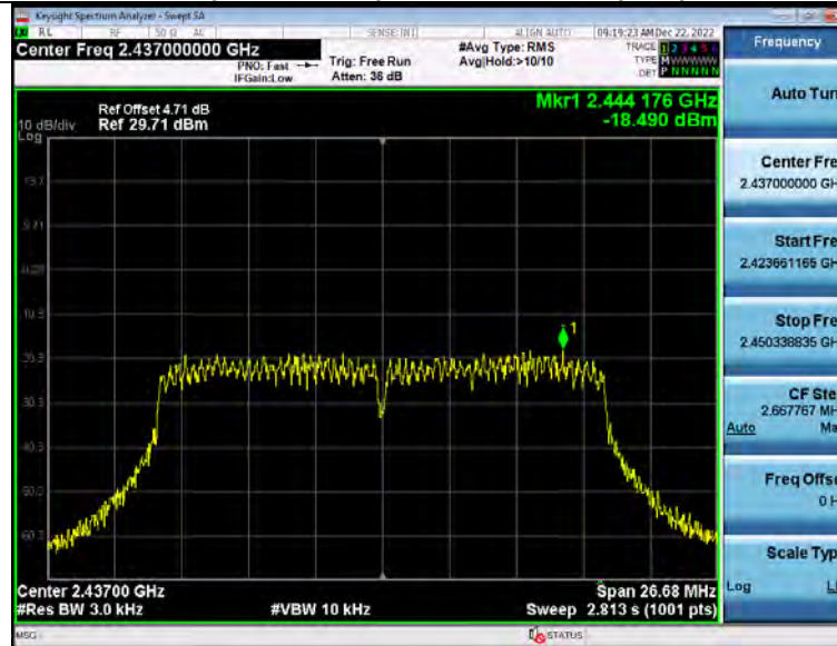
Power Spectral Density 2_4GWiFi_802_11n(HT20)_2437
