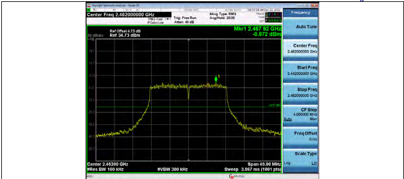
2_Bandedge 2_4GWiFi_NVNT_ANT1_802_11g_2462
