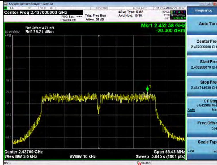
Power Spectral Density 2_4GWiFi_802_11n(HT40)_2437
