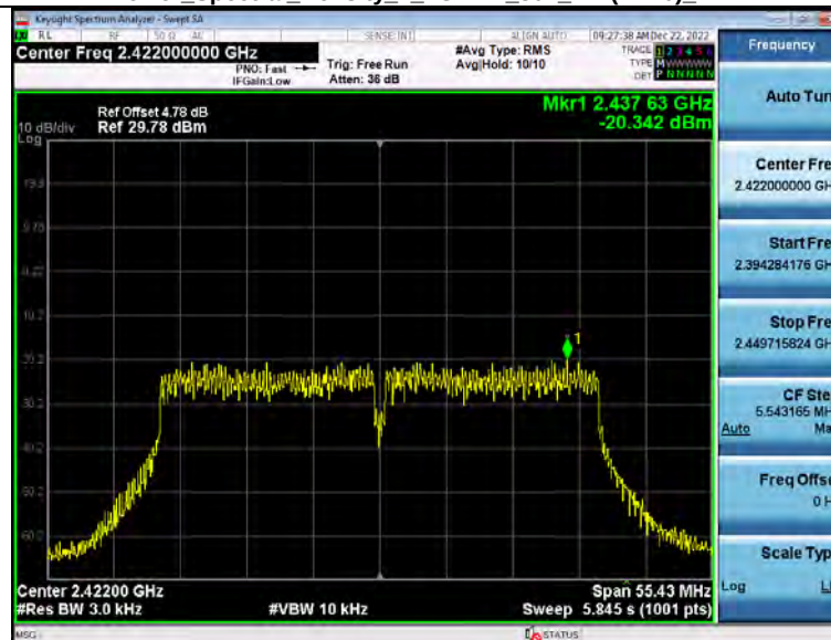
Power Spectral Density 2_4GWiFi_802_11n(HT40)_2422
