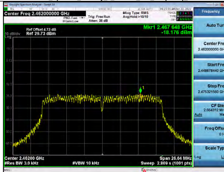
Power Spectral Density 2_4GWiFi_802_11n(HT20)_2462
