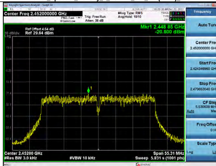
Power Spectral Density 2_4GWiFi_802_11n(HT40)_2452
