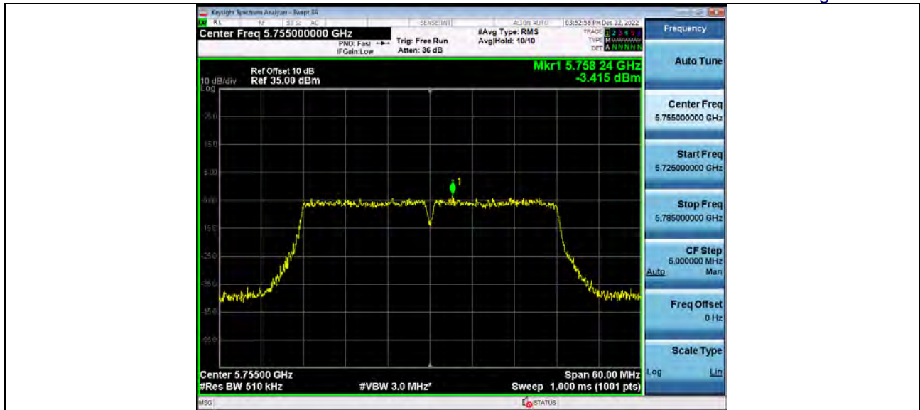
Power_Spectral_Density_5_8WiFi_802_11n(HT40)_5795_40M
