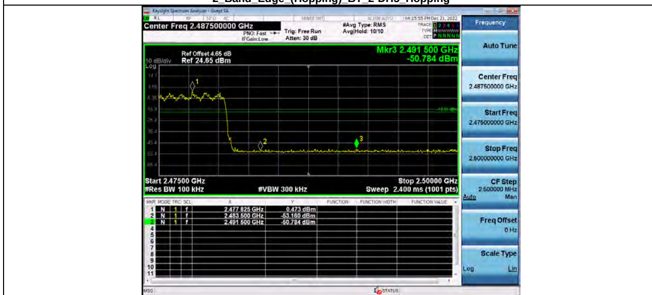
2_Band_Edge (Hopping) BT 2-DH5 Hopping
