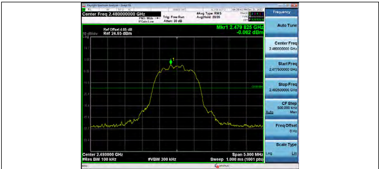
2_Bandedge_BT_3-DH5_2480
